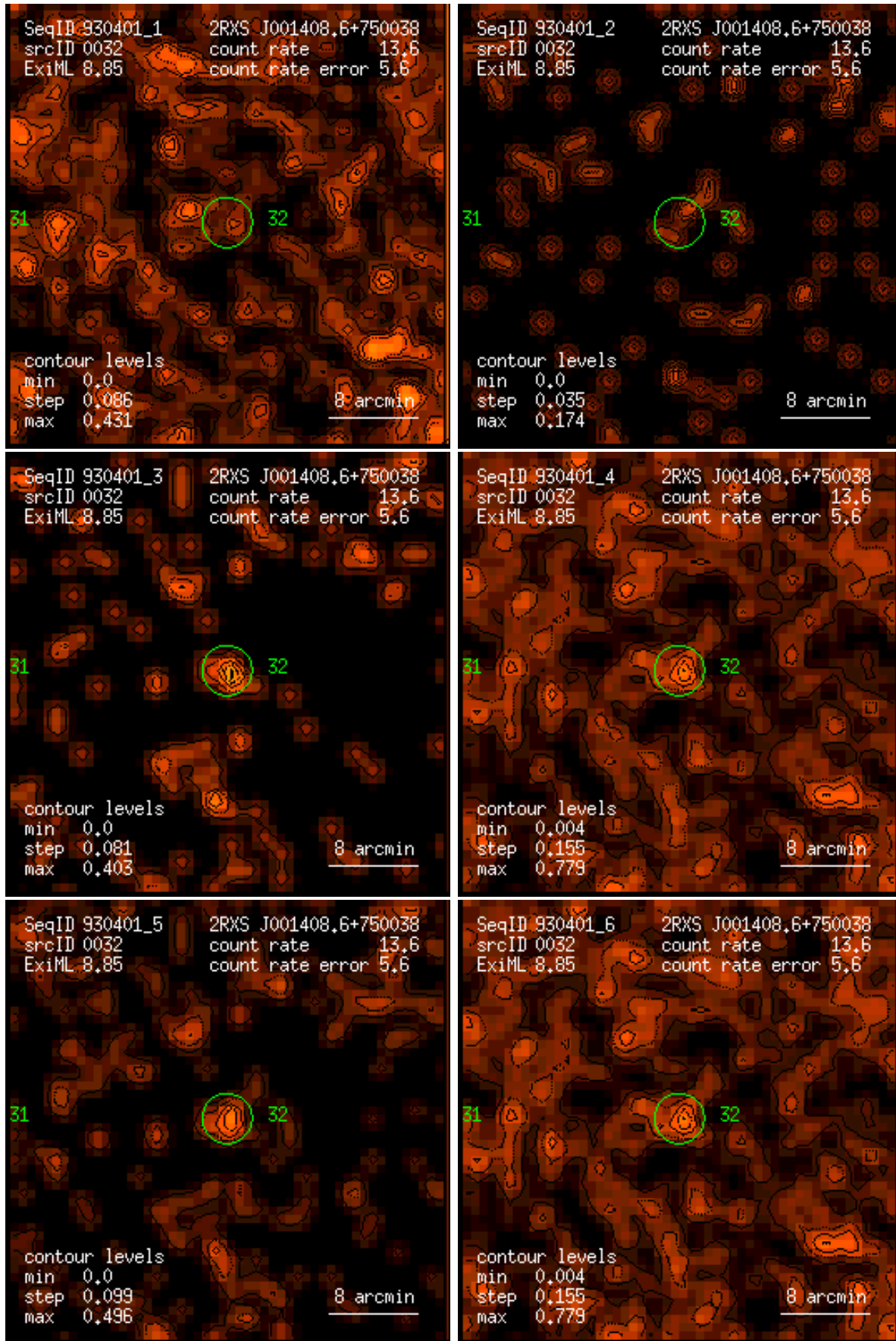
Figure 32: RASS 930401: detection 0032: band rate images, Gaussian filter: (1) PSPC channels 11 – 41, (2) 52 – 90, (3) 91 – 201, (4) 11 – 235, (5) 52 – 201, (6) 11 – 201. Broad band rates in counts/ks. Band rate contour levels in counts/ks/arcmin 2 .
