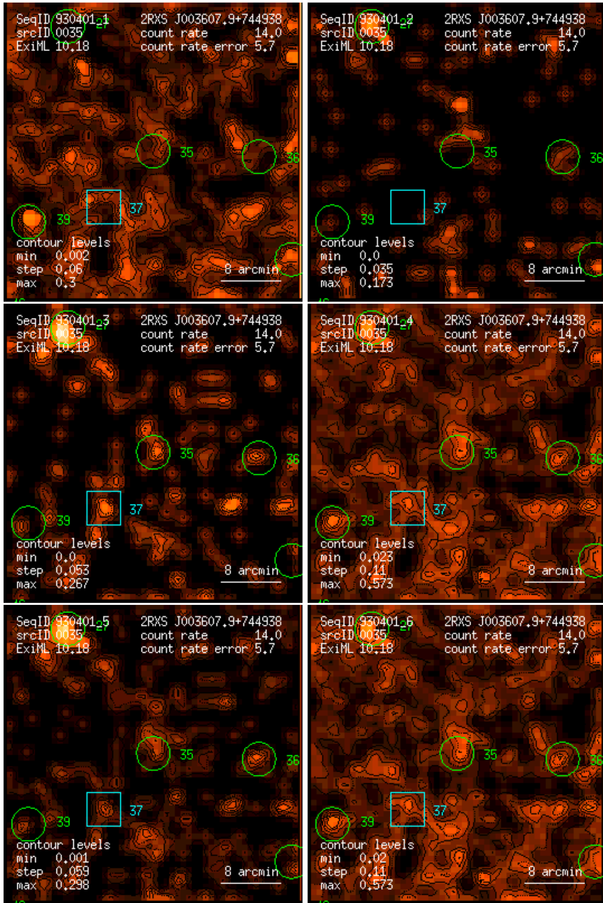
Figure 35: RASS 930401: detection 0035: band rate images, Gaussian filter: (1) PSPC channels 11 – 41, (2) 52 – 90, (3) 91 – 201, (4) 11 – 235, (5) 52 – 201, (6) 11 – 201. Broad band rates in counts/ks. Band rate contour levels in counts/ks/arcmin 2 .
