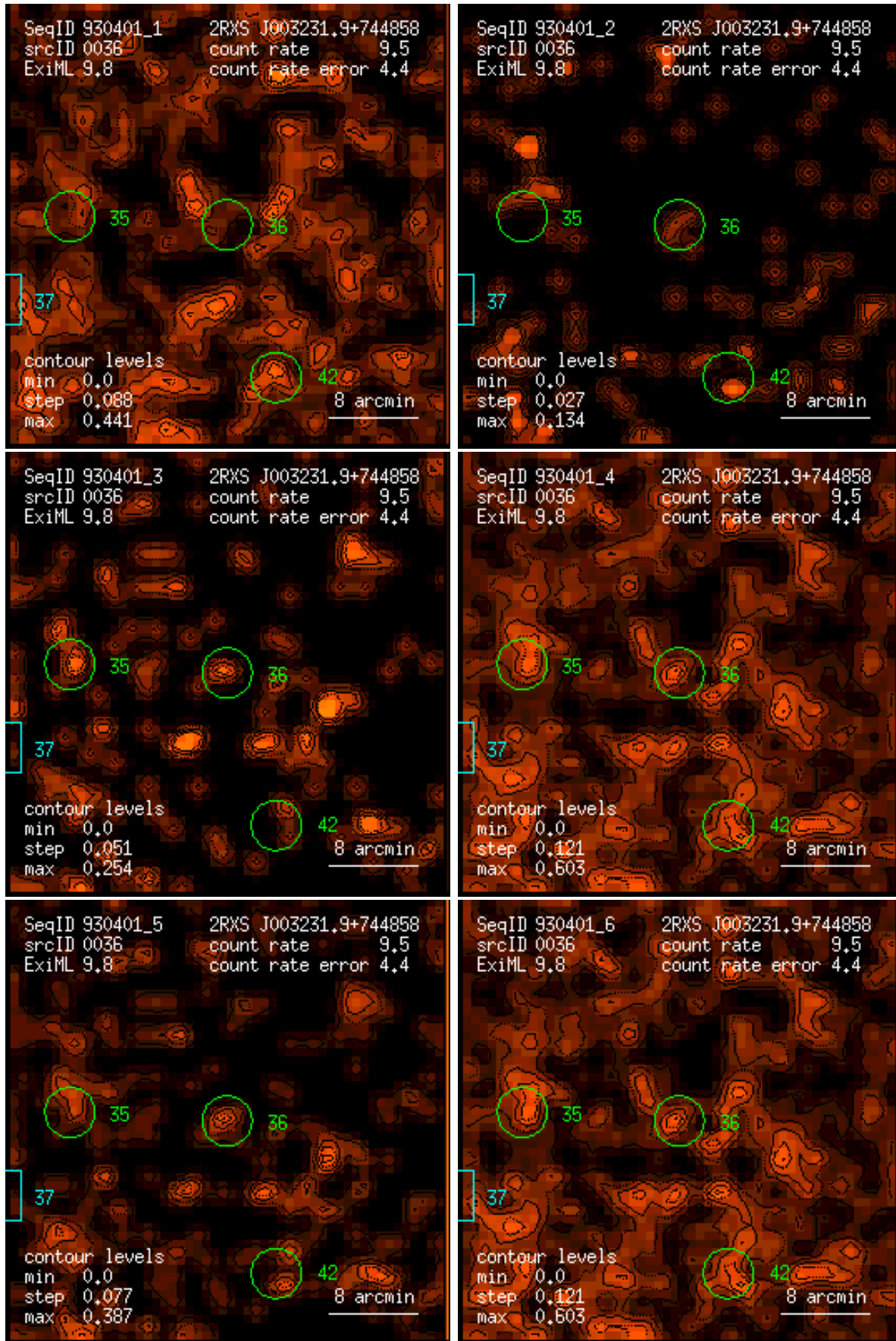
Figure 36: RASS 930401: detection 0036: band rate images, Gaussian filter: (1) PSPC channels 11 – 41, (2) 52 – 90, (3) 91 – 201, (4) 11 – 235, (5) 52 – 201, (6) 11 – 201. Broad band rates in counts/ks. Band rate contour levels in counts/ks/arcmin 2 .
