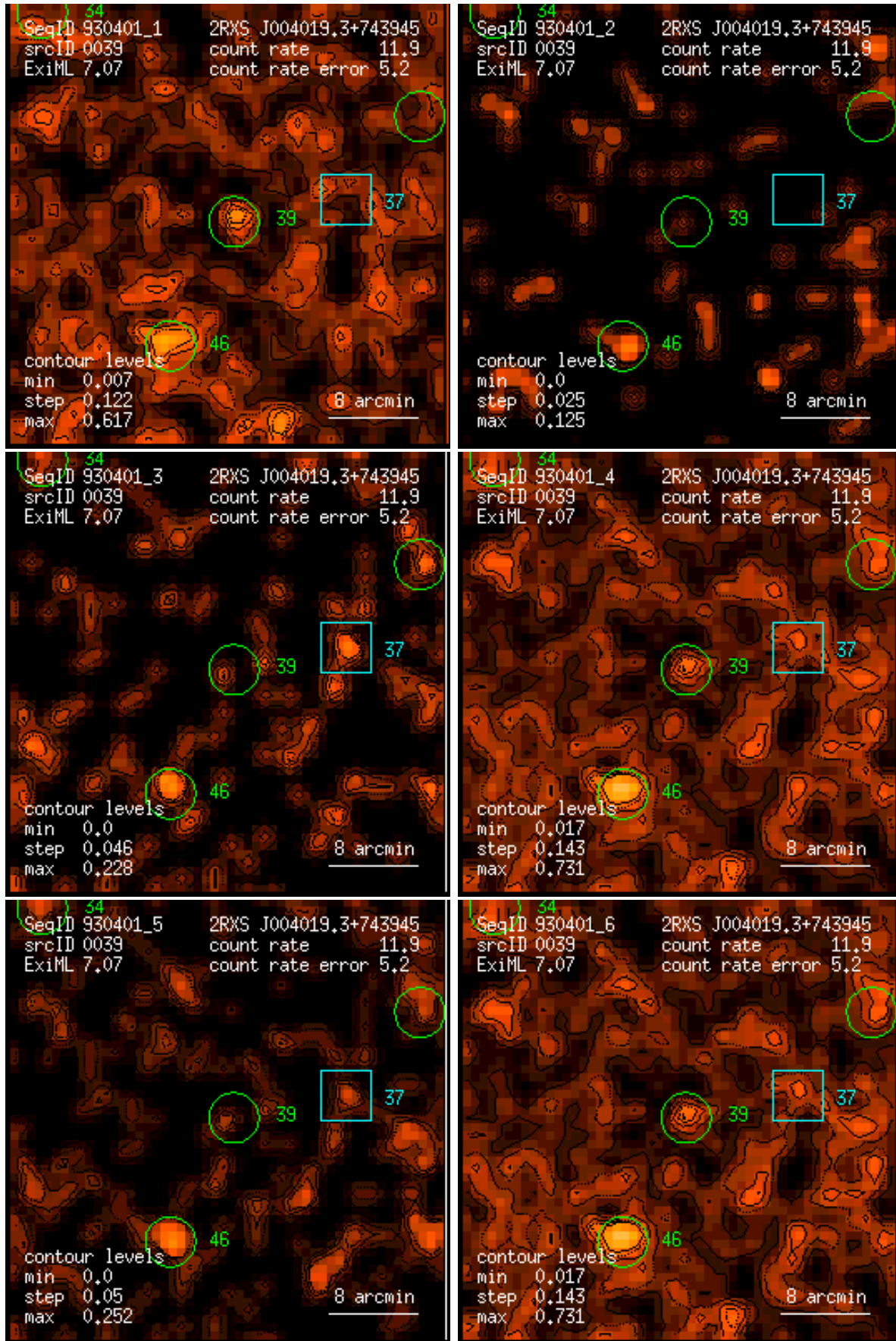
Figure 39: RASS 930401: detection 0039: band rate images, Gaussian filter: (1) PSPC channels 11 – 41, (2) 52 – 90, (3) 91 – 201, (4) 11 – 235, (5) 52 – 201, (6) 11 – 201. Broad band rates in counts/ks. Band rate contour levels in counts/ks/arcmin 2 .
