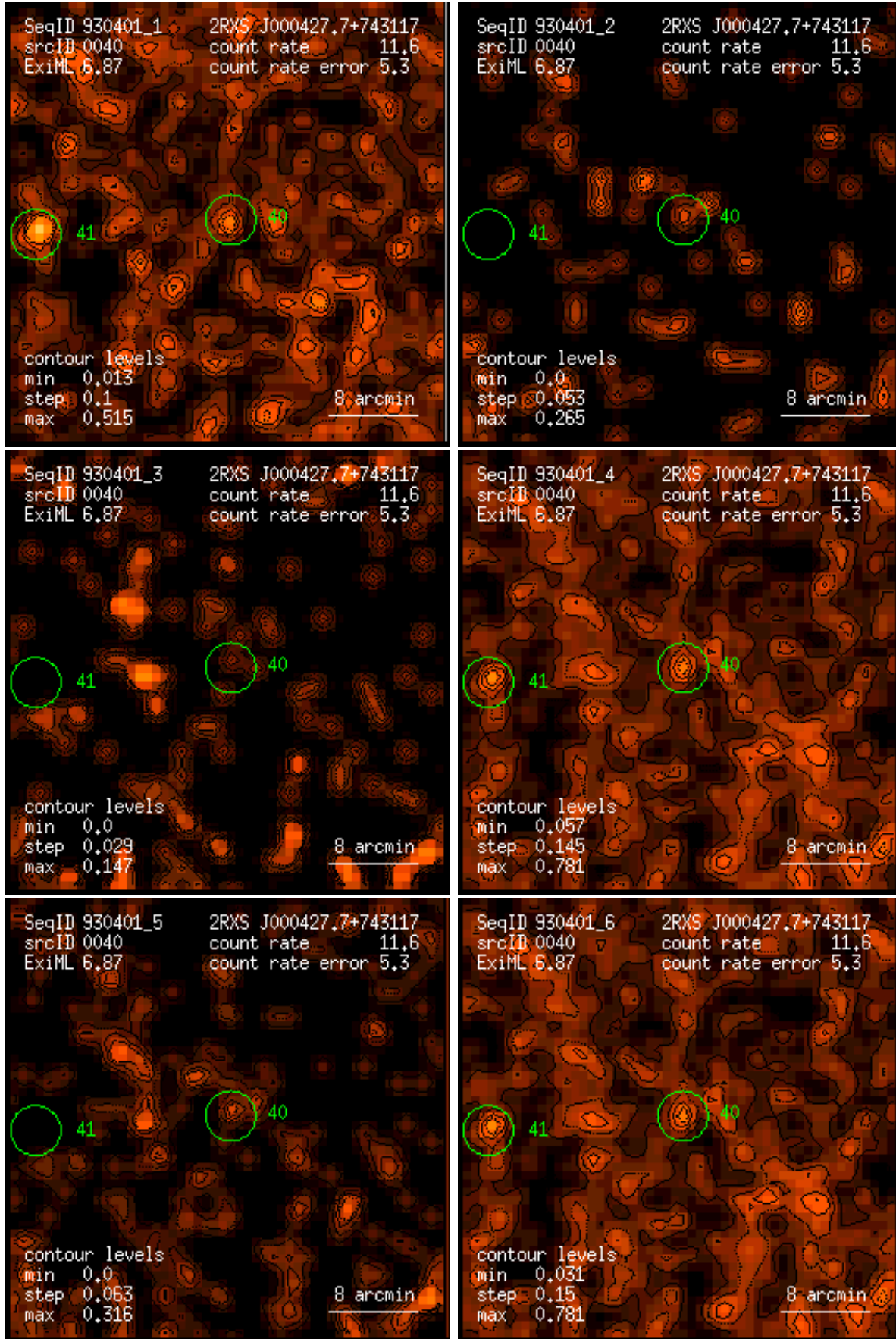
Figure 40: RASS 930401: detection 0040: band rate images, Gaussian filter: (1) PSPC channels 11 – 41, (2) 52 – 90, (3) 91 – 201, (4) 11 – 235, (5) 52 – 201, (6) 11 – 201. Broad band rates in counts/ks. Band rate contour levels in counts/ks/arcmin 2 .
