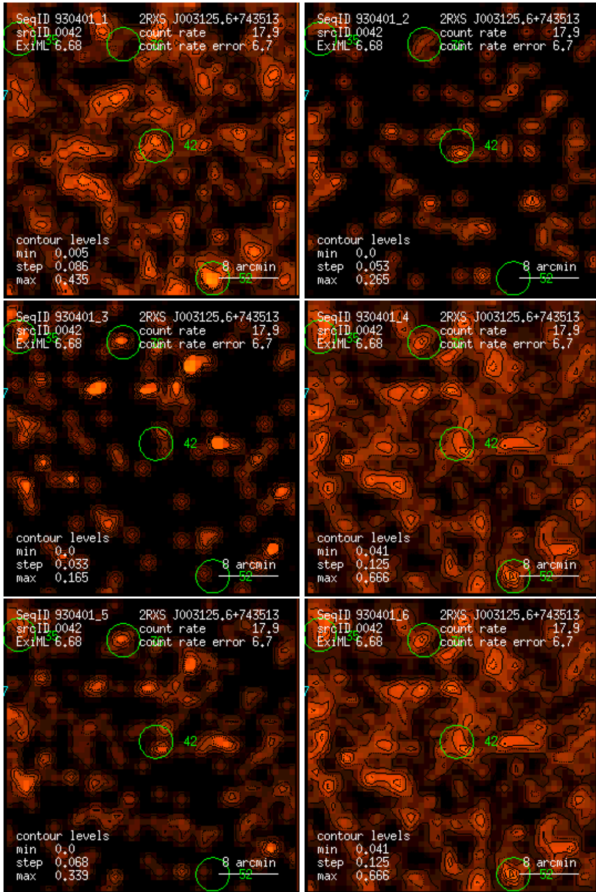
Figure 42: RASS 930401: detection 0042: band rate images, Gaussian filter: (1) PSPC channels 11 – 41, (2) 52 – 90, (3) 91 – 201, (4) 11 – 235, (5) 52 – 201, (6) 11 – 201. Broad band rates in counts/ks. Band rate contour levels in counts/ks/arcmin 2 .
