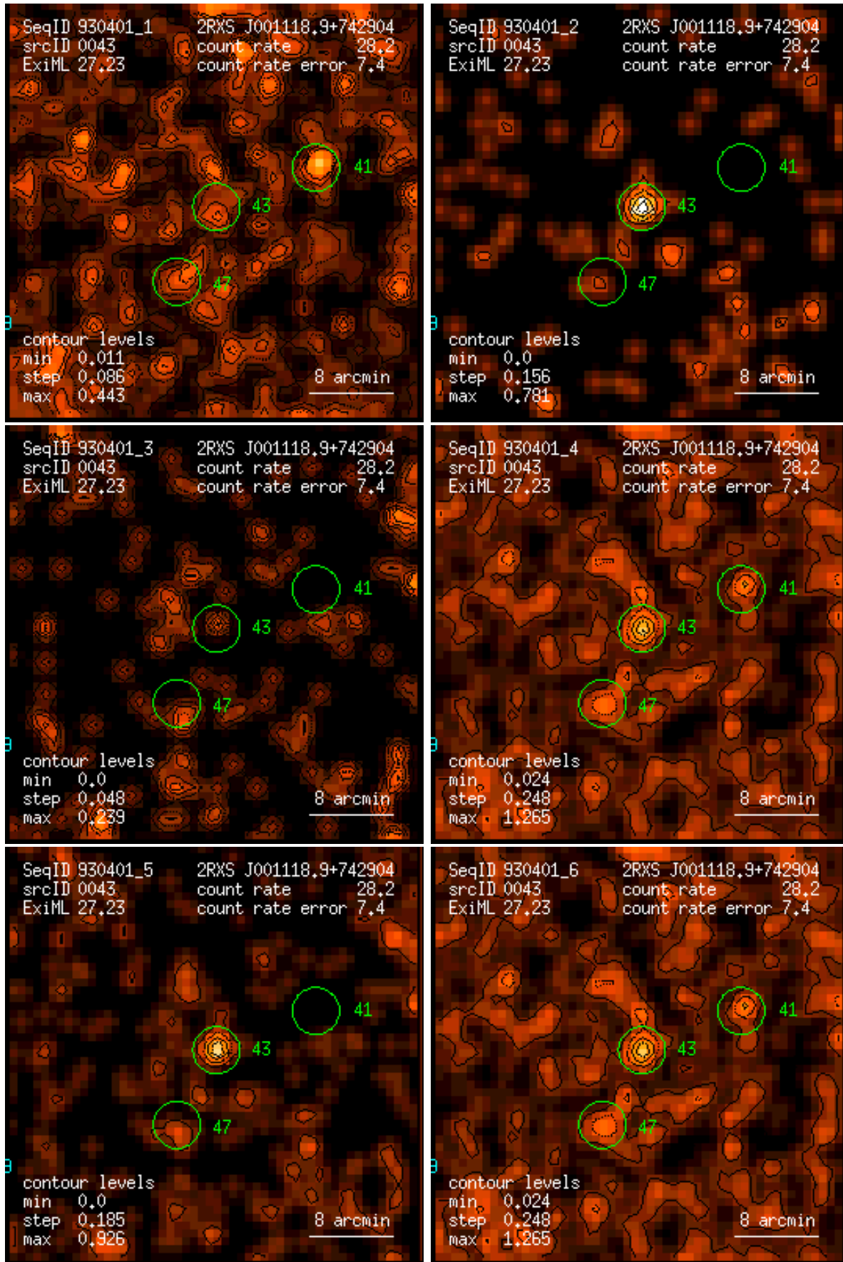
Figure 43: RASS 930401: detection 0043: band rate images, Gaussian filter: (1) PSPC channels 11 – 41, (2) 52 – 90, (3) 91 – 201, (4) 11 – 235, (5) 52 – 201, (6) 11 – 201. Broad band rates in counts/ks. Band rate contour levels in counts/ks/arcmin 2 .
