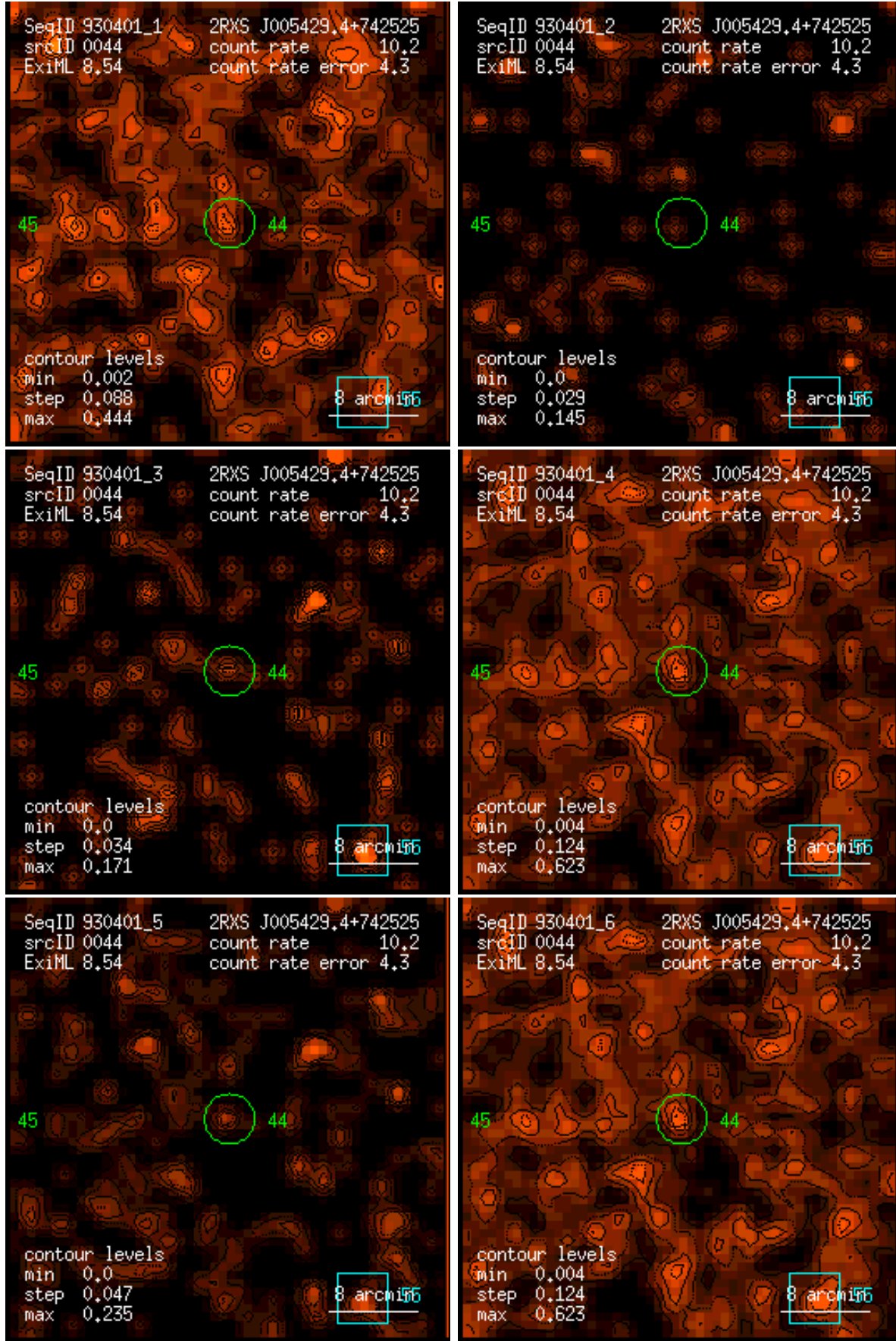
Figure 44: RASS 930401: detection 0044: band rate images, Gaussian filter: (1) PSPC channels 11 – 41, (2) 52 – 90, (3) 91 – 201, (4) 11 – 235, (5) 52 – 201, (6) 11 – 201. Broad band rates in counts/ks. Band rate contour levels in counts/ks/arcmin 2 .
