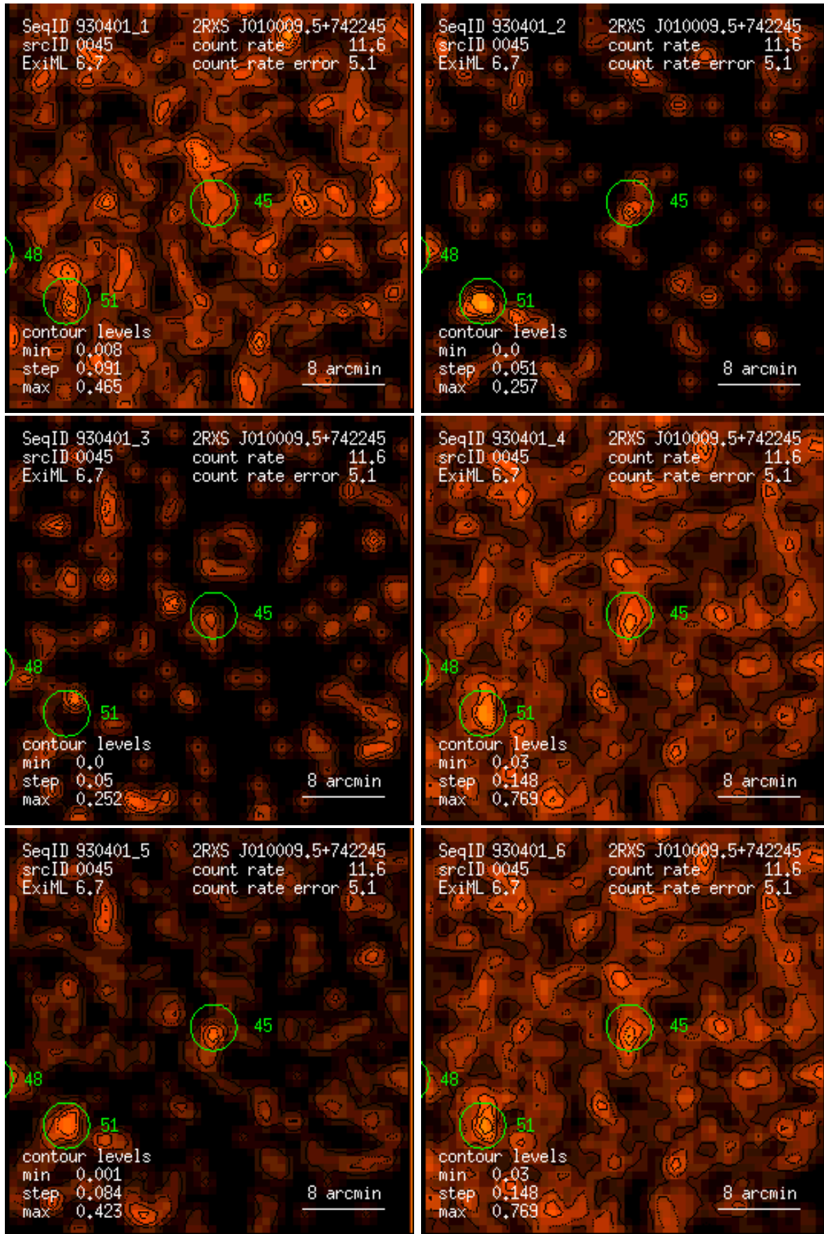
Figure 45: RASS 930401: detection 0045: band rate images, Gaussian filter: (1) PSPC channels 11 – 41, (2) 52 – 90, (3) 91 – 201, (4) 11 – 235, (5) 52 – 201, (6) 11 – 201. Broad band rates in counts/ks. Band rate contour levels in counts/ks/arcmin 2 .
