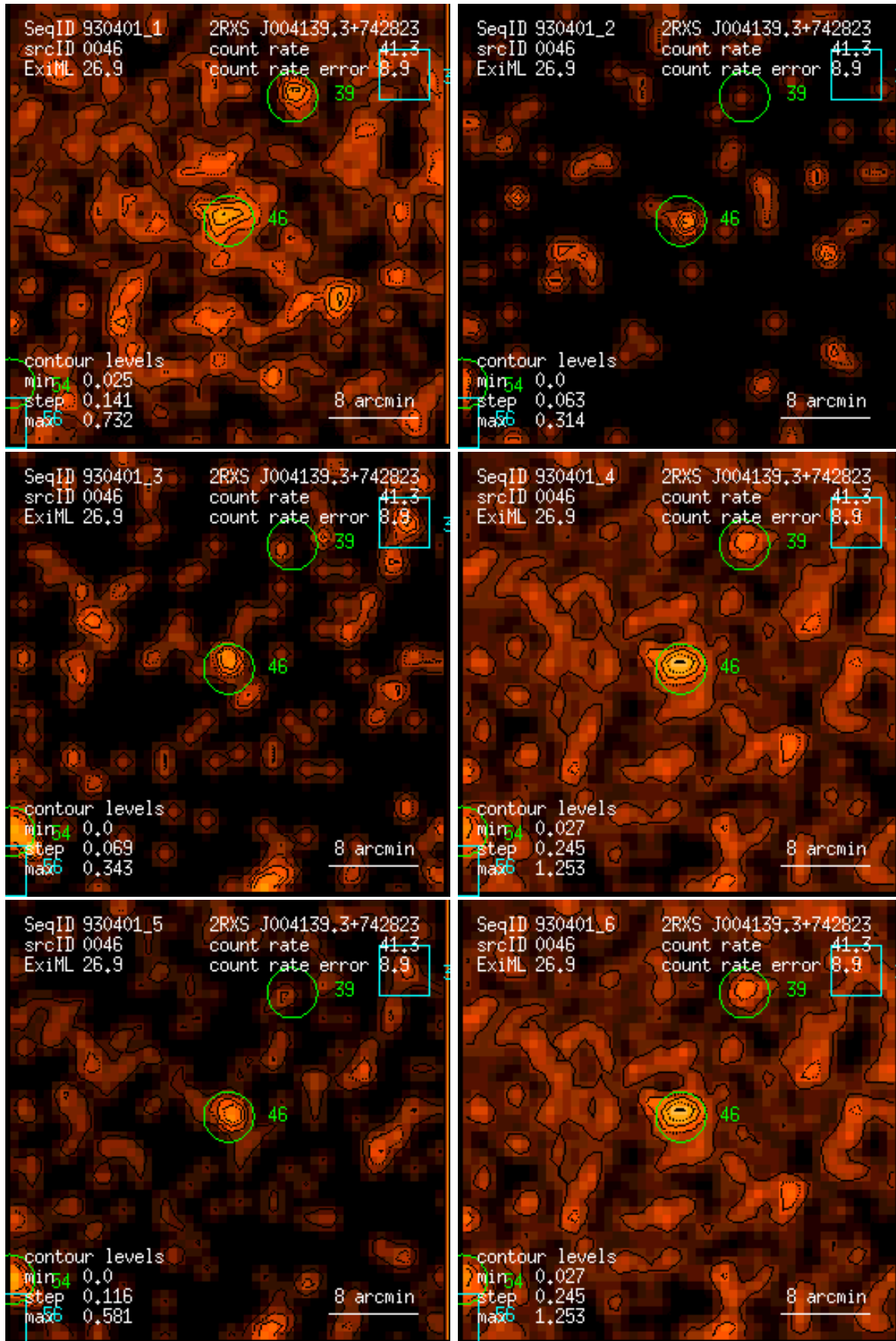
Figure 46: RASS 930401: detection 0046: band rate images, Gaussian filter: (1) PSPC channels 11 – 41, (2) 52 – 90, (3) 91 – 201, (4) 11 – 235, (5) 52 – 201, (6) 11 – 201. Broad band rates in counts/ks. Band rate contour levels in counts/ks/arcmin 2 .
