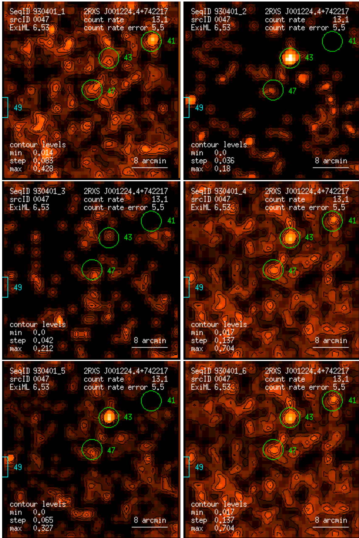
Figure 47: RASS 930401: detection 0047: band rate images, Gaussian filter: (1) PSPC channels 11 – 41, (2) 52 – 90, (3) 91 – 201, (4) 11 – 235, (5) 52 – 201, (6) 11 – 201. Broad band rates in counts/ks. Band rate contour levels in counts/ks/arcmin 2 .
