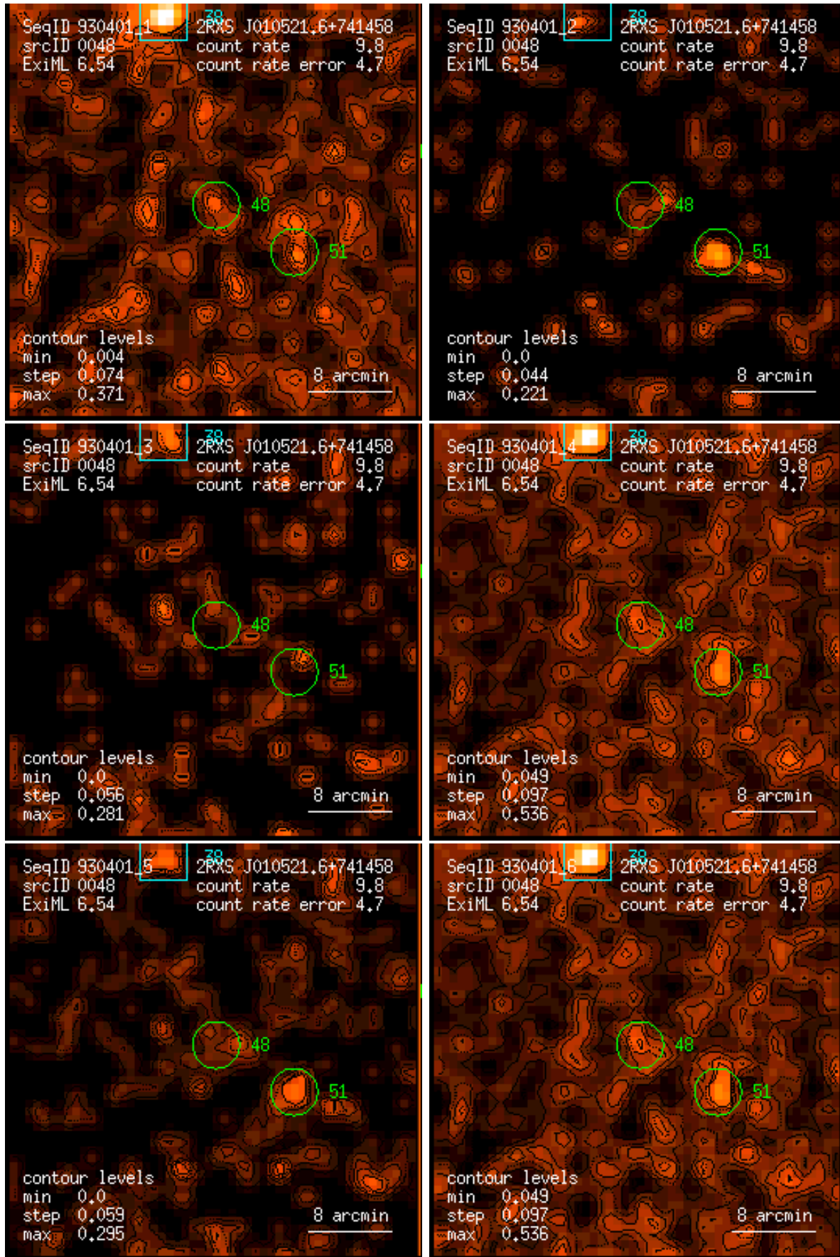
Figure 48: RASS 930401: detection 0048: band rate images, Gaussian filter: (1) PSPC channels 11 – 41, (2) 52 – 90, (3) 91 – 201, (4) 11 – 235, (5) 52 – 201, (6) 11 – 201. Broad band rates in counts/ks. Band rate contour levels in counts/ks/arcmin 2 .
