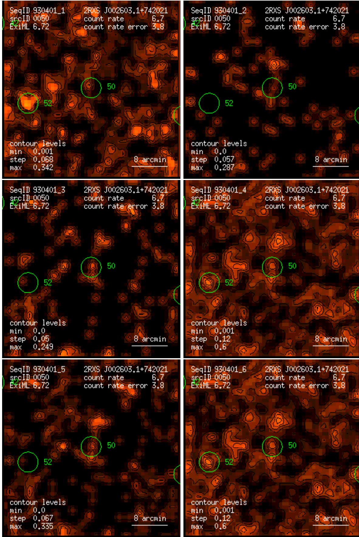
Figure 50: RASS 930401: detection 0050: band rate images, Gaussian filter: (1) PSPC channels 11 – 41, (2) 52 – 90, (3) 91 – 201, (4) 11 – 235, (5) 52 – 201, (6) 11 – 201. Broad band rates in counts/ks. Band rate contour levels in counts/ks/arcmin 2 .
