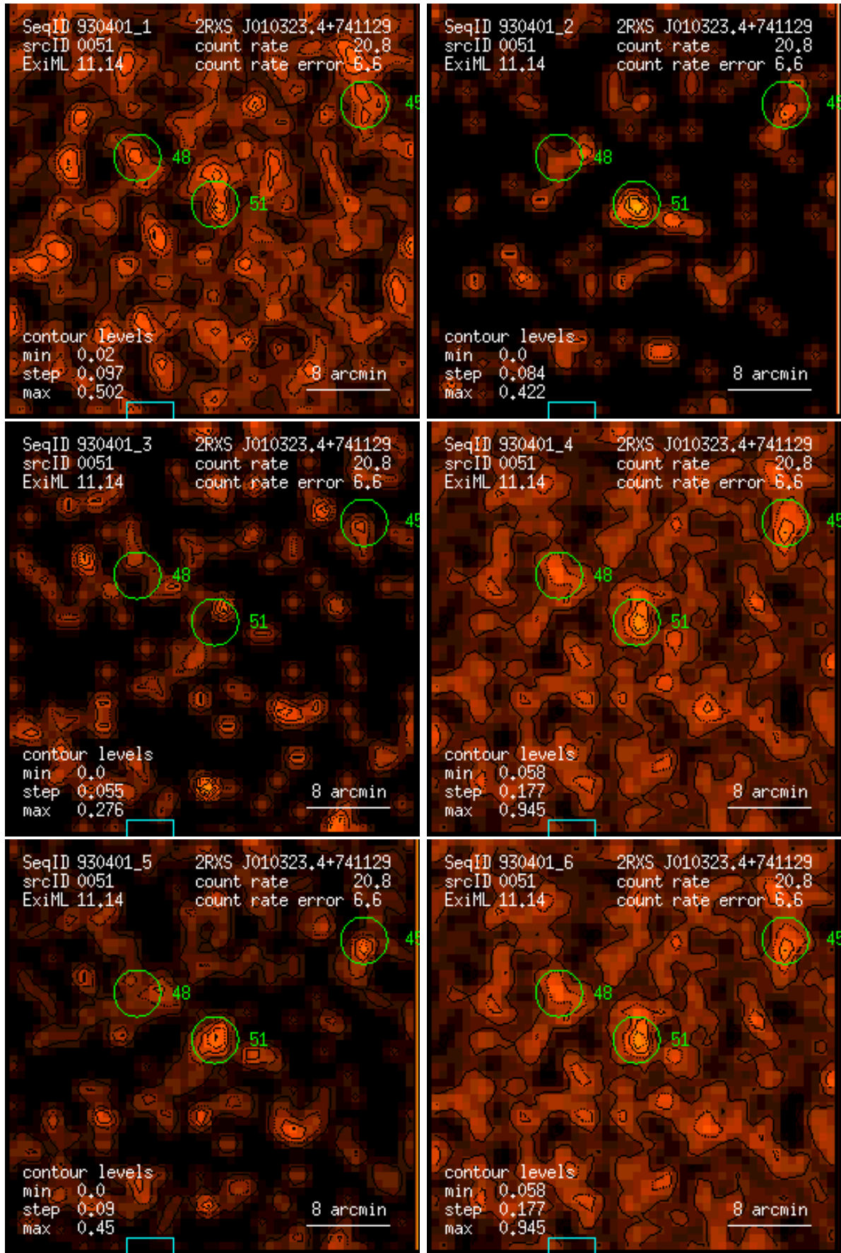
Figure 51: RASS 930401: detection 0051: band rate images, Gaussian filter: (1) PSPC channels 11 – 41, (2) 52 – 90, (3) 91 – 201, (4) 11 – 235, (5) 52 – 201, (6) 11 – 201. Broad band rates in counts/ks. Band rate contour levels in counts/ks/arcmin 2 .
