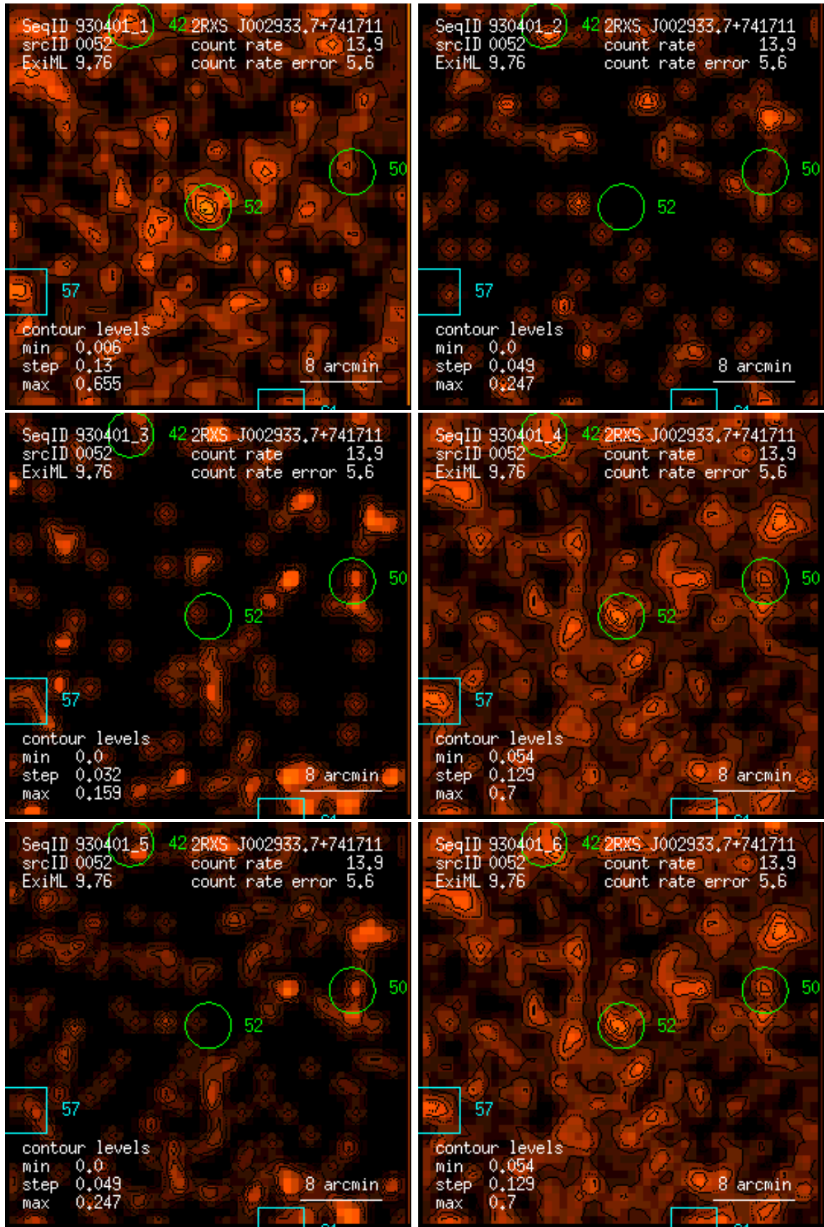
Figure 52: RASS 930401: detection 0052: band rate images, Gaussian filter: (1) PSPC channels 11 – 41, (2) 52 – 90, (3) 91 – 201, (4) 11 – 235, (5) 52 – 201, (6) 11 – 201. Broad band rates in counts/ks. Band rate contour levels in counts/ks/arcmin 2 .
