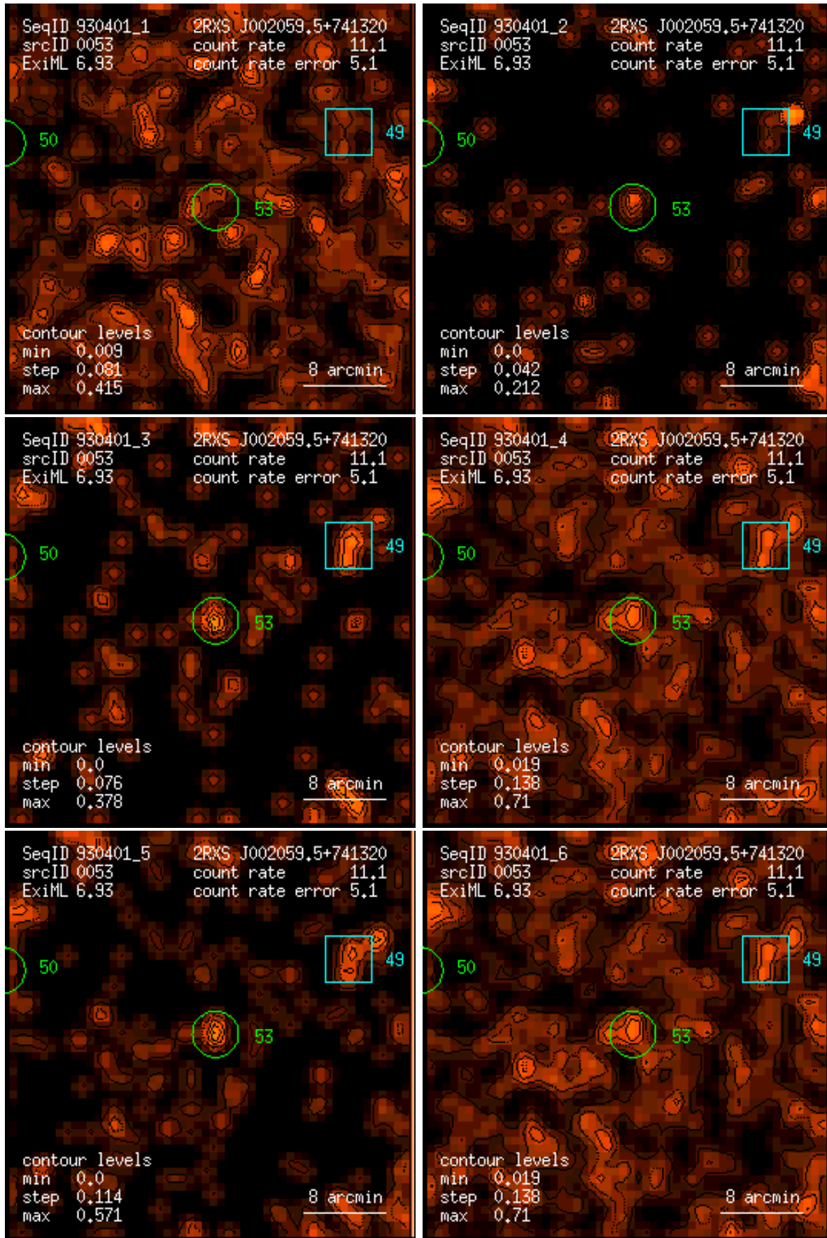
Figure 53: RASS 930401: detection 0053: band rate images, Gaussian filter: (1) PSPC channels 11 – 41, (2) 52 – 90, (3) 91 – 201, (4) 11 – 235, (5) 52 – 201, (6) 11 – 201. Broad band rates in counts/ks. Band rate contour levels in counts/ks/arcmin 2 .
