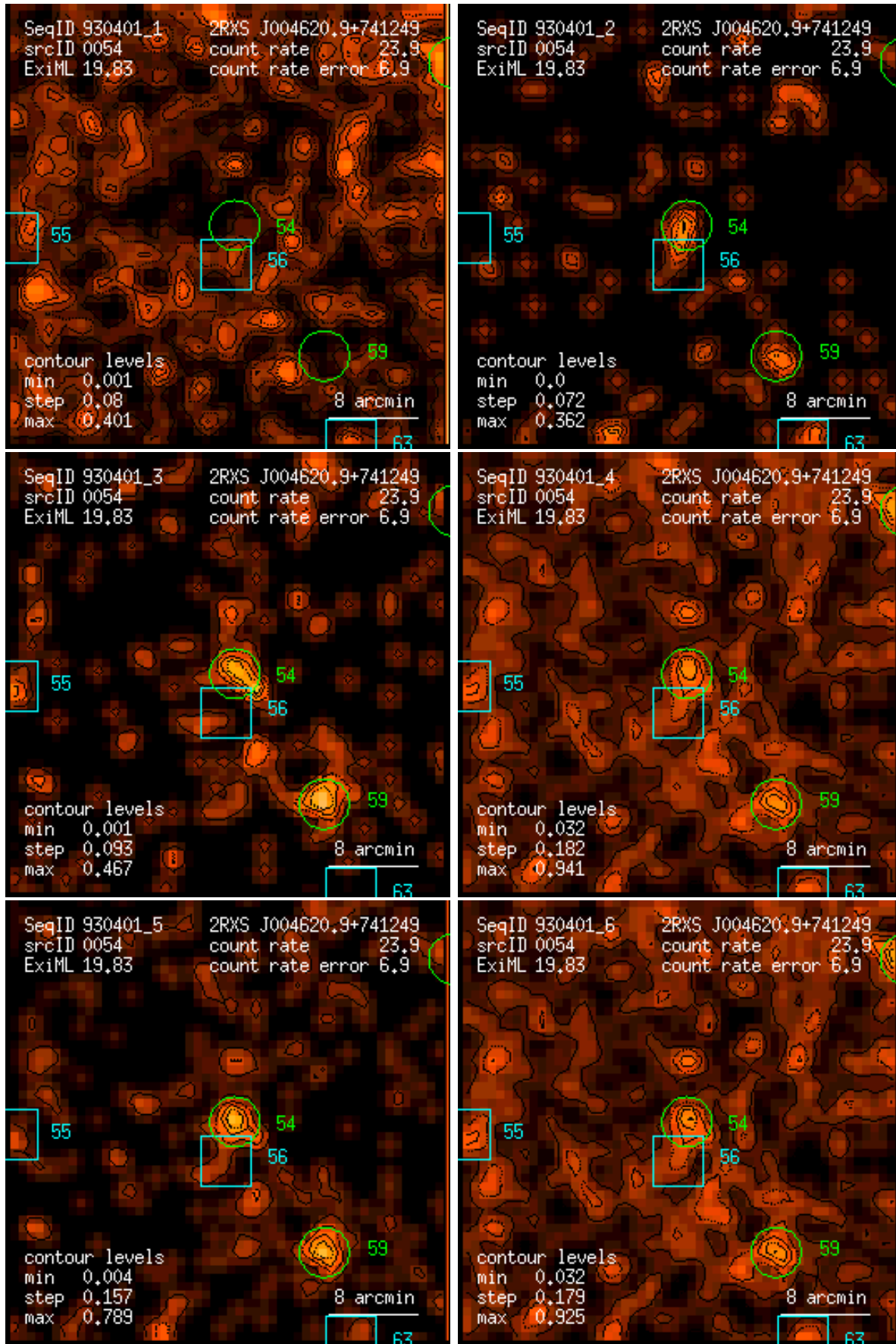
Figure 54: RASS 930401: detection 0054: band rate images, Gaussian filter: (1) PSPC channels 11 – 41, (2) 52 – 90, (3) 91 – 201, (4) 11 – 235, (5) 52 – 201, (6) 11 – 201. Broad band rates in counts/ks. Band rate contour levels in counts/ks/arcmin 2 .
