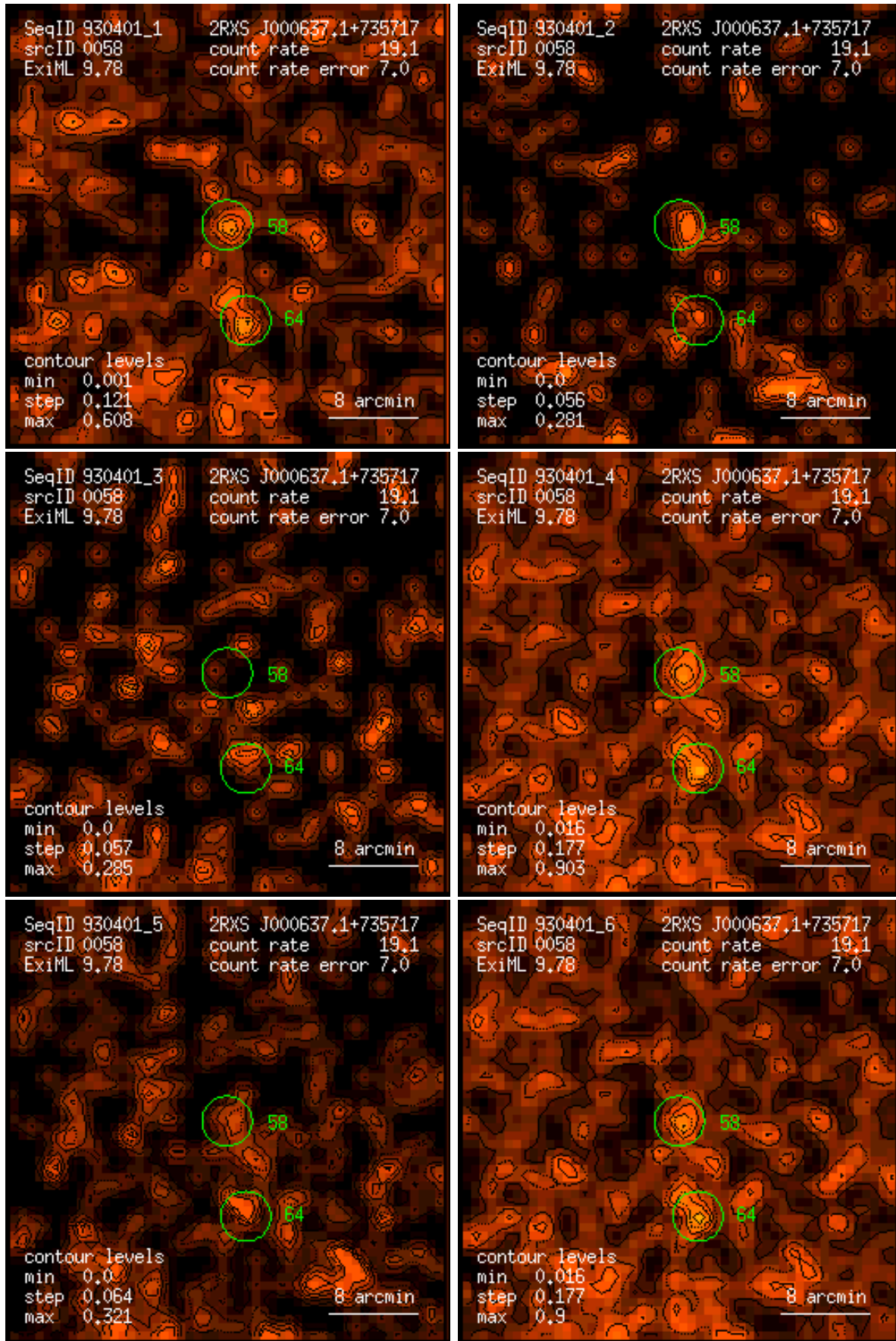
Figure 58: RASS 930401: detection 0058: band rate images, Gaussian filter: (1) PSPC channels 11 – 41, (2) 52 – 90, (3) 91 – 201, (4) 11 – 235, (5) 52 – 201, (6) 11 – 201. Broad band rates in counts/ks. Band rate contour levels in counts/ks/arcmin 2 .
