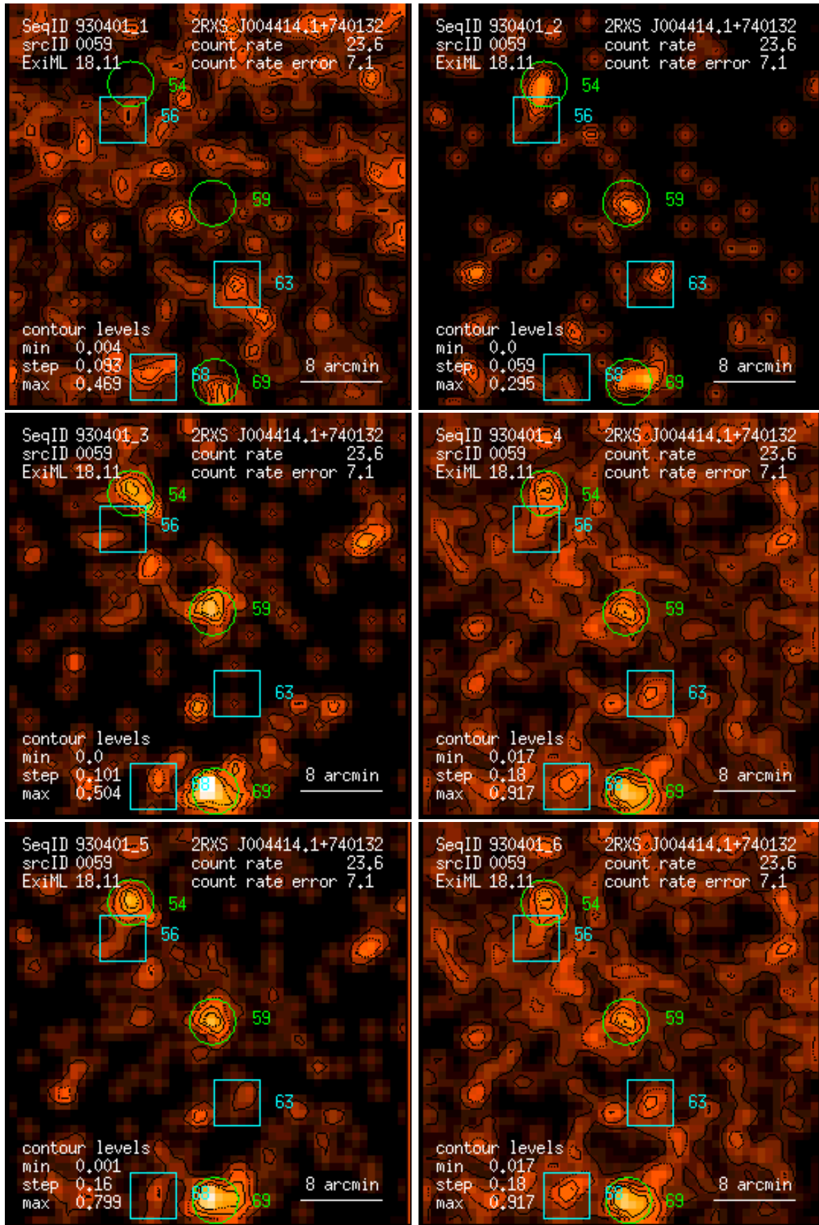
Figure 59: RASS 930401: detection 0059: band rate images, Gaussian filter: (1) PSPC channels 11 – 41, (2) 52 – 90, (3) 91 – 201, (4) 11 – 235, (5) 52 – 201, (6) 11 – 201. Broad band rates in counts/ks. Band rate contour levels in counts/ks/arcmin 2 .
