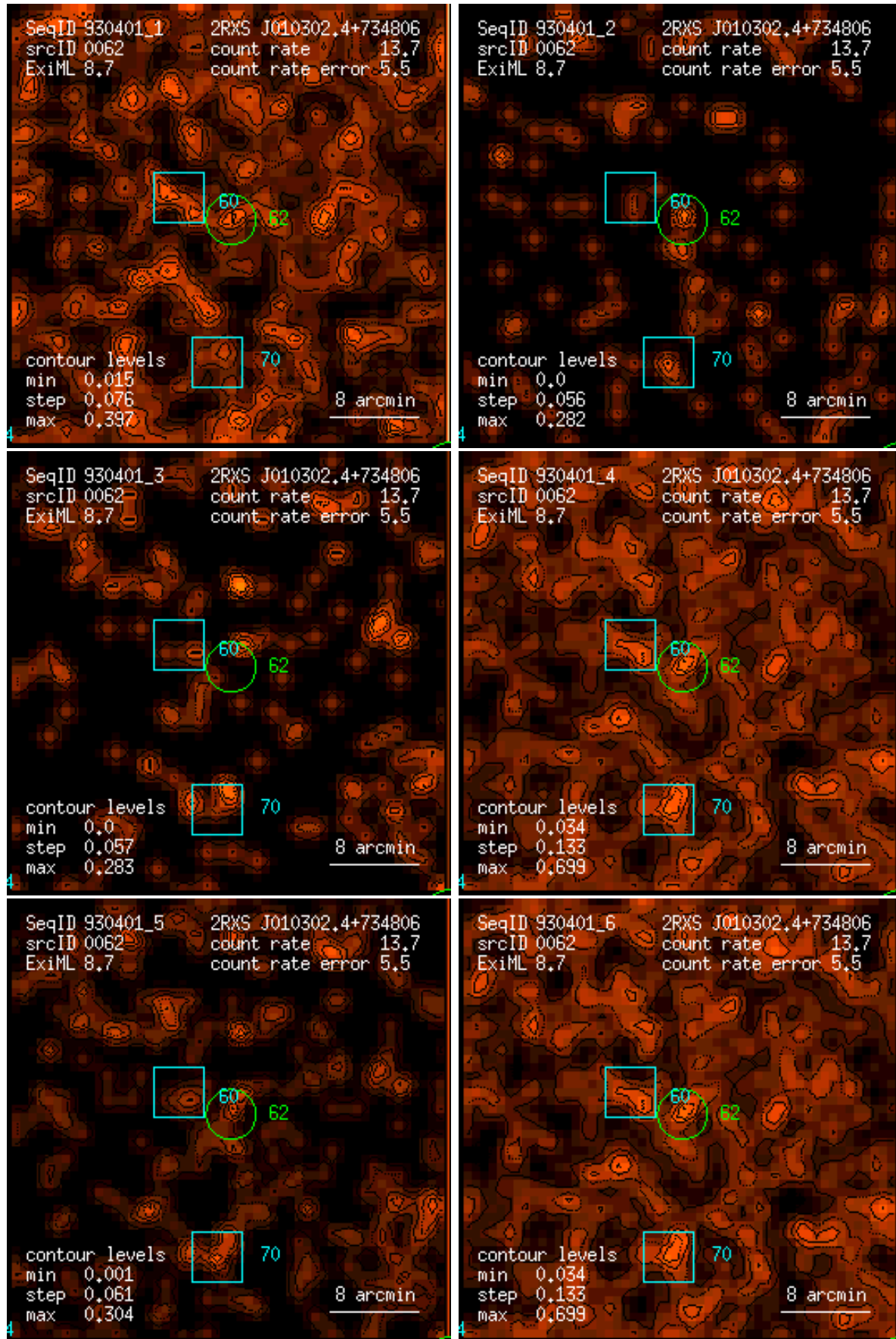
Figure 62: RASS 930401: detection 0062: band rate images, Gaussian filter: (1) PSPC channels 11 – 41, (2) 52 – 90, (3) 91 – 201, (4) 11 – 235, (5) 52 – 201, (6) 11 – 201. Broad band rates in counts/ks. Band rate contour levels in counts/ks/arcmin 2 .
