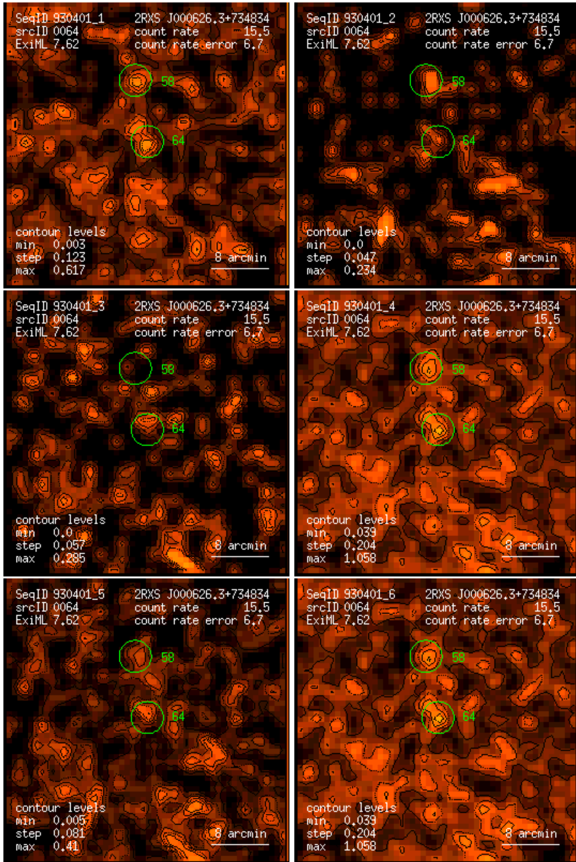
Figure 64: RASS 930401: detection 0064: band rate images, Gaussian filter: (1) PSPC channels 11 – 41, (2) 52 – 90, (3) 91 – 201, (4) 11 – 235, (5) 52 – 201, (6) 11 – 201. Broad band rates in counts/ks. Band rate contour levels in counts/ks/arcmin 2 .
