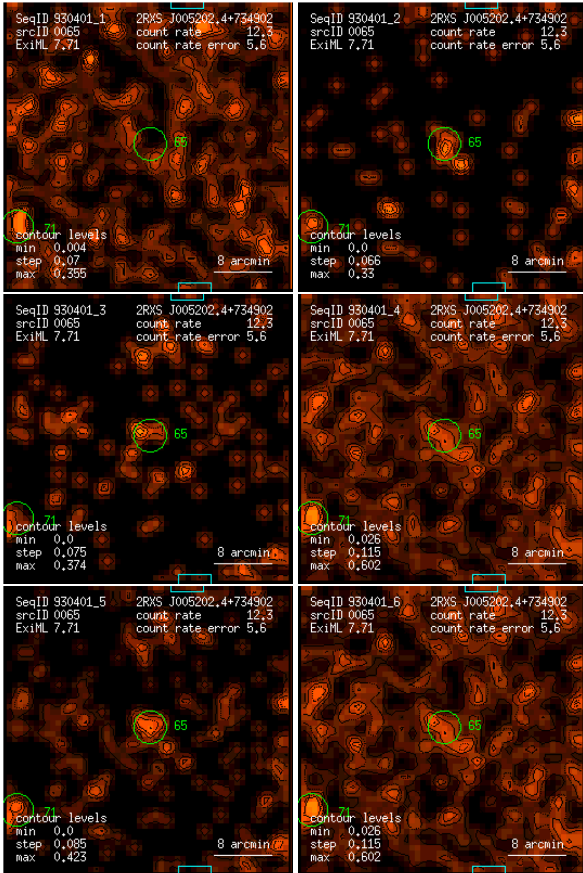
Figure 65: RASS 930401: detection 0065: band rate images, Gaussian filter: (1) PSPC channels 11 – 41, (2) 52 – 90, (3) 91 – 201, (4) 11 – 235, (5) 52 – 201, (6) 11 – 201. Broad band rates in counts/ks. Band rate contour levels in counts/ks/arcmin 2 .
