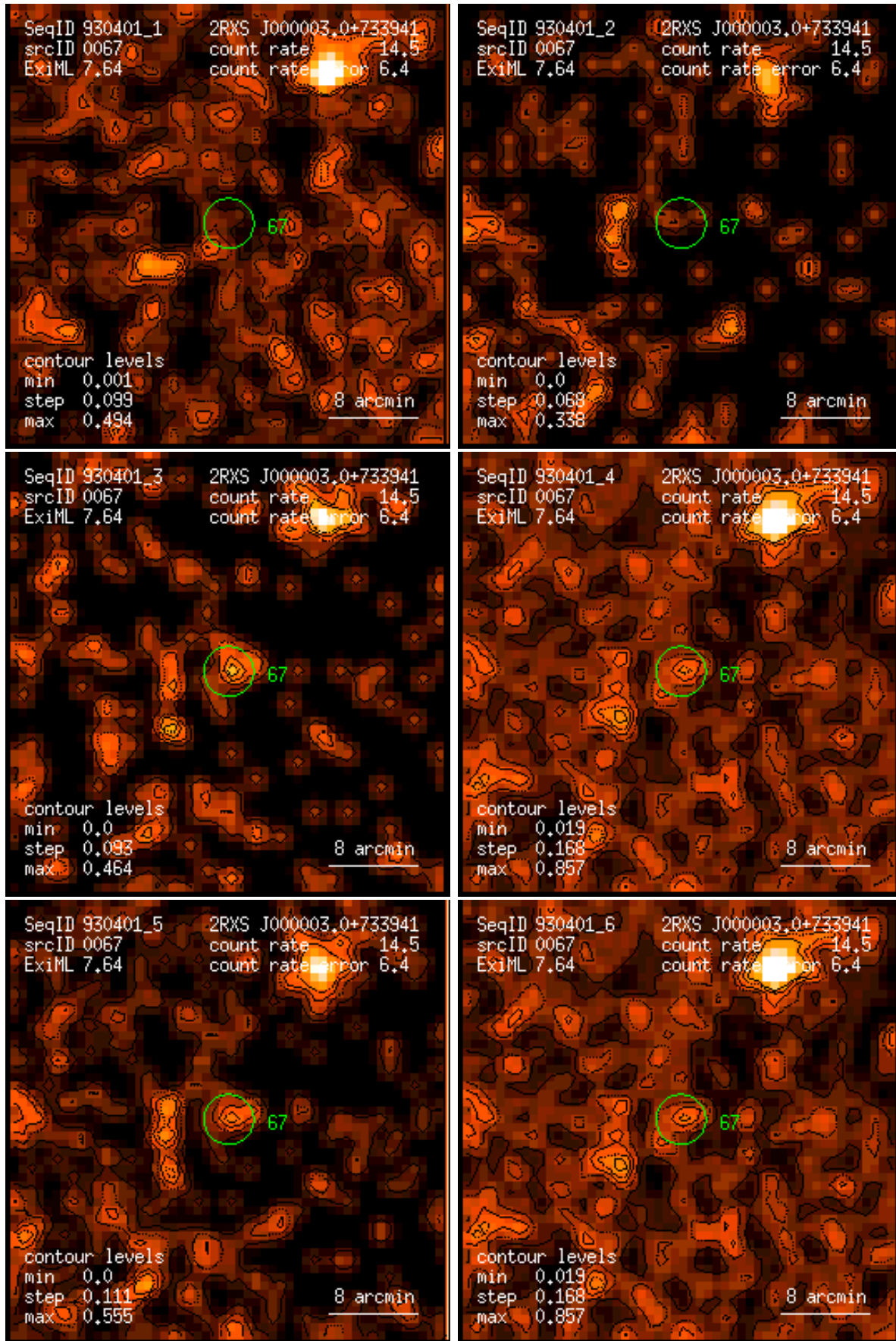
Figure 67: RASS 930401: detection 0067: band rate images, Gaussian filter: (1) PSPC channels 11 – 41, (2) 52 – 90, (3) 91 – 201, (4) 11 – 235, (5) 52 – 201, (6) 11 – 201. Broad band rates in counts/ks. Band rate contour levels in counts/ks/arcmin 2 .
