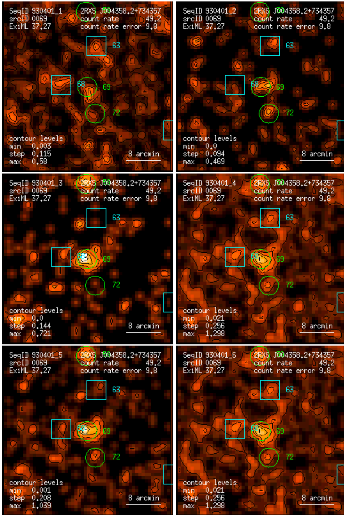
Figure 69: RASS 930401: detection 0069: band rate images, Gaussian filter: (1) PSPC channels 11 – 41, (2) 52 – 90, (3) 91 – 201, (4) 11 – 235, (5) 52 – 201, (6) 11 – 201. Broad band rates in counts/ks. Band rate contour levels in counts/ks/arcmin 2 .
