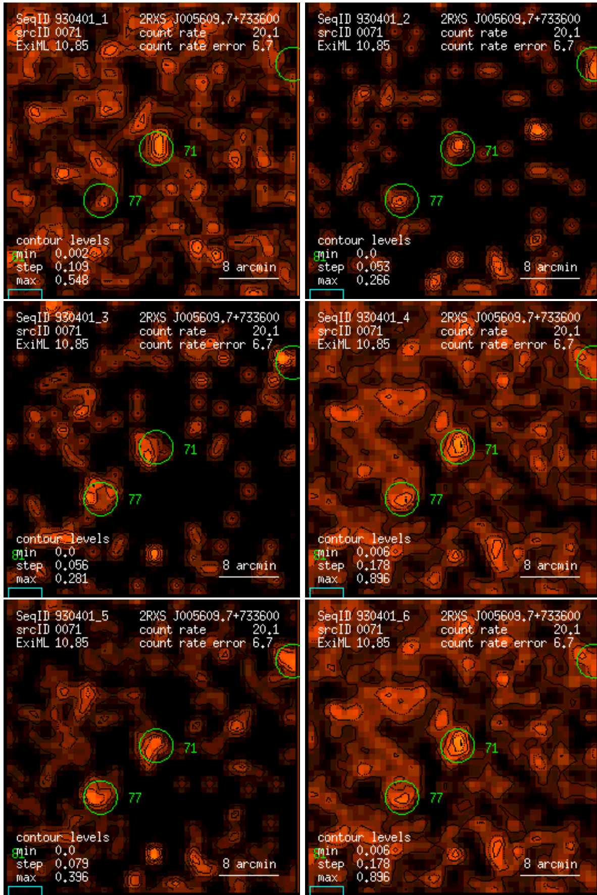
Figure 71: RASS 930401: detection 0071: band rate images, Gaussian filter: (1) PSPC channels 11 – 41, (2) 52 – 90, (3) 91 – 201, (4) 11 – 235, (5) 52 – 201, (6) 11 – 201. Broad band rates in counts/ks. Band rate contour levels in counts/ks/arcmin 2 .
