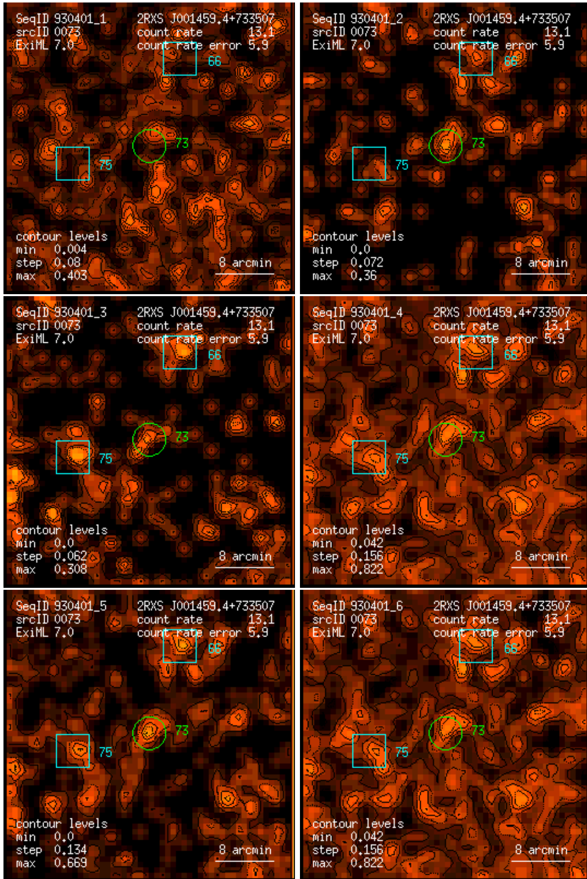
Figure 73: RASS 930401: detection 0073: band rate images, Gaussian filter: (1) PSPC channels 11 – 41, (2) 52 – 90, (3) 91 – 201, (4) 11 – 235, (5) 52 – 201, (6) 11 – 201. Broad band rates in counts/ks. Band rate contour levels in counts/ks/arcmin 2 .
