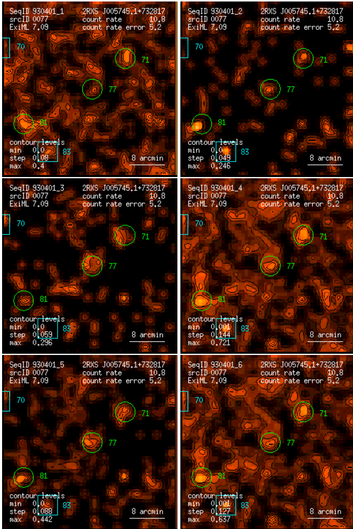
Figure 77: RASS 930401: detection 0077: band rate images, Gaussian filter: (1) PSPC channels 11 – 41, (2) 52 – 90, (3) 91 – 201, (4) 11 – 235, (5) 52 – 201, (6) 11 – 201. Broad band rates in counts/ks. Band rate contour levels in counts/ks/arcmin 2 .
