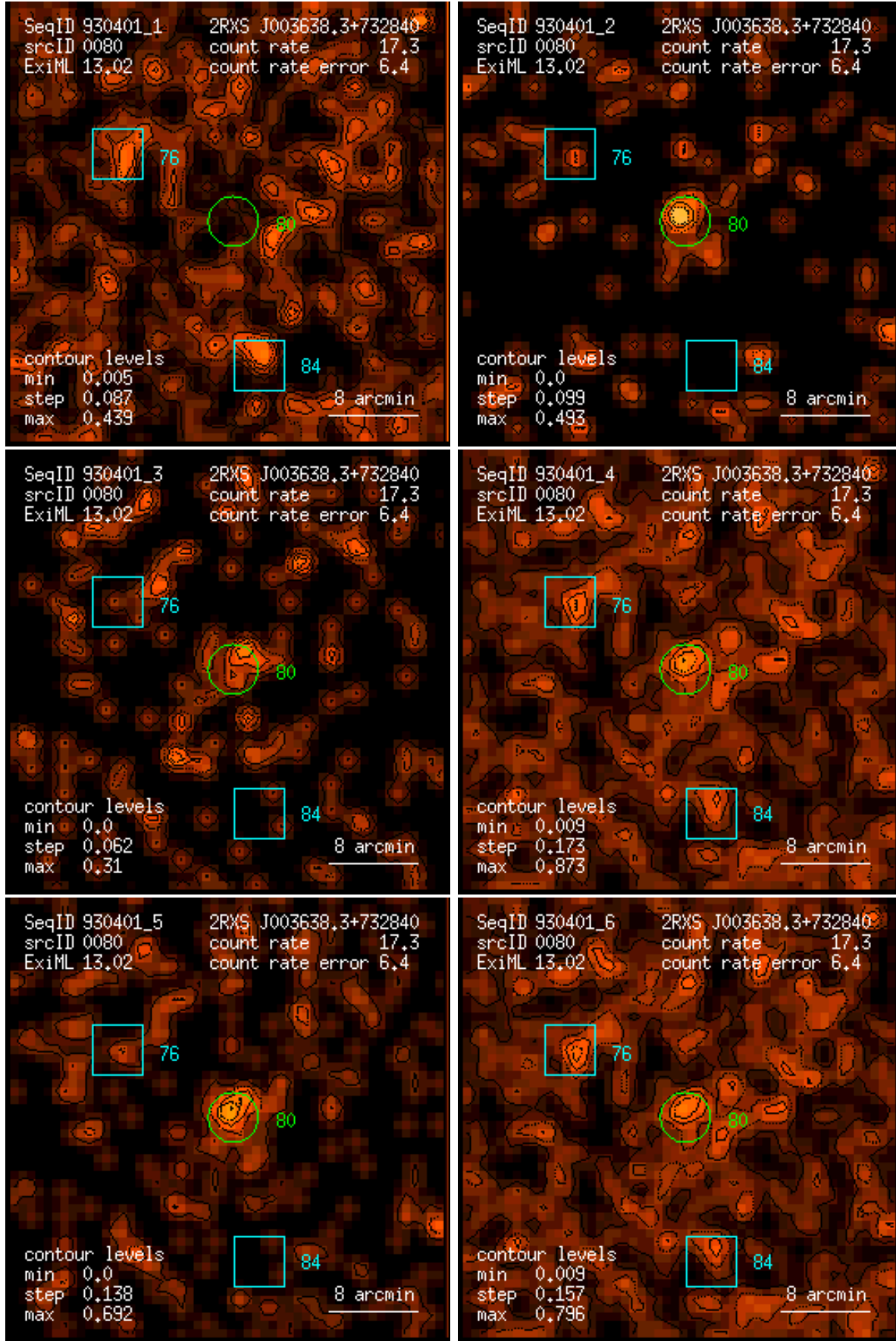
Figure 80: RASS 930401: detection 0080: band rate images, Gaussian filter: (1) PSPC channels 11 – 41, (2) 52 – 90, (3) 91 – 201, (4) 11 – 235, (5) 52 – 201, (6) 11 – 201. Broad band rates in counts/ks. Band rate contour levels in counts/ks/arcmin 2 .
