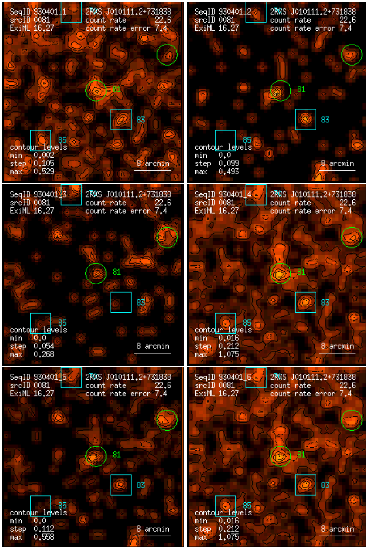
Figure 81: RASS 930401: detection 0081: band rate images, Gaussian filter: (1) PSPC channels 11 – 41, (2) 52 – 90, (3) 91 – 201, (4) 11 – 235, (5) 52 – 201, (6) 11 – 201. Broad band rates in counts/ks. Band rate contour levels in counts/ks/arcmin 2 .
