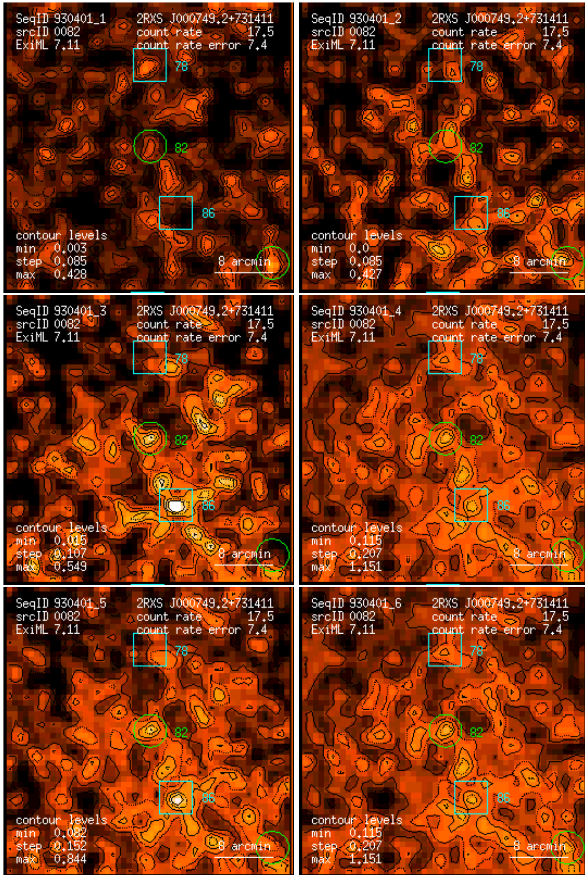
Figure 82: RASS 930401: detection 0082: band rate images, Gaussian filter: (1) PSPC channels 11 – 41, (2) 52 – 90, (3) 91 – 201, (4) 11 – 235, (5) 52 – 201, (6) 11 – 201. Broad band rates in counts/ks. Band rate contour levels in counts/ks/arcmin 2 .
