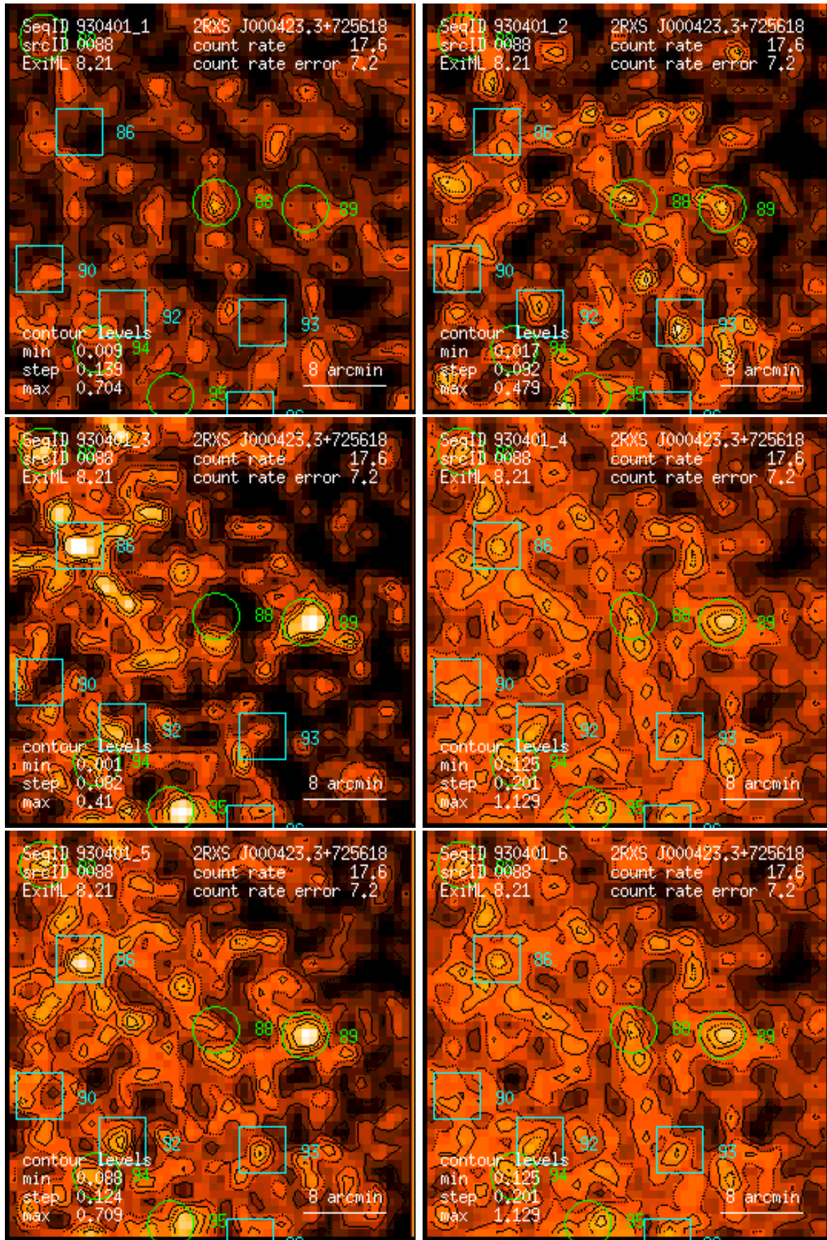
Figure 88: RASS 930401: detection 0088: band rate images, Gaussian filter: (1) PSPC channels 11 – 41, (2) 52 – 90, (3) 91 – 201, (4) 11 – 235, (5) 52 – 201, (6) 11 – 201. Broad band rates in counts/ks. Band rate contour levels in counts/ks/arcmin 2 .
