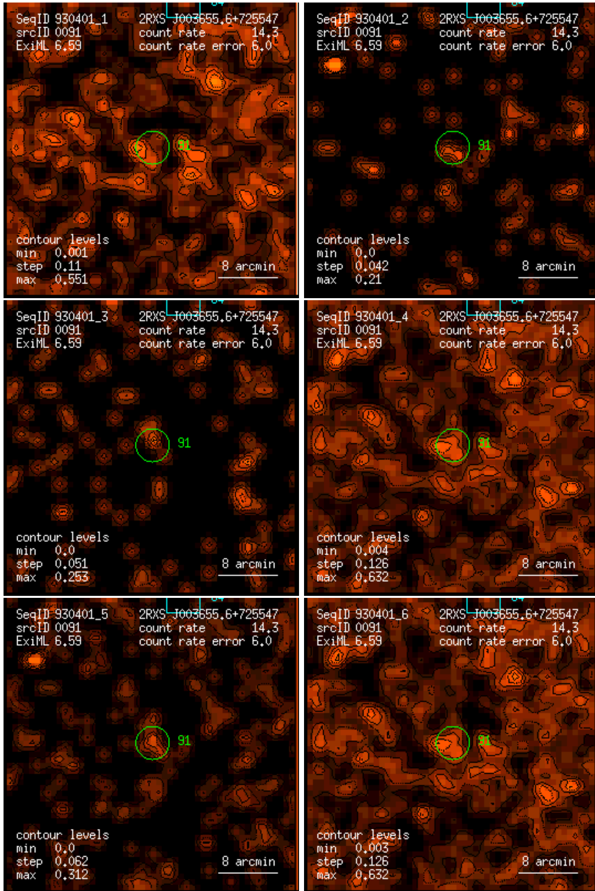
Figure 91: RASS 930401: detection 0091: band rate images, Gaussian filter: (1) PSPC channels 11 – 41, (2) 52 – 90, (3) 91 – 201, (4) 11 – 235, (5) 52 – 201, (6) 11 – 201. Broad band rates in counts/ks. Band rate contour levels in counts/ks/arcmin 2 .
