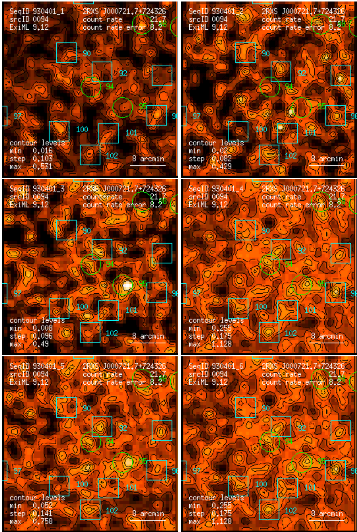
Figure 94: RASS 930401: detection 0094: band rate images, Gaussian filter: (1) PSPC channels 11 – 41, (2) 52 – 90, (3) 91 – 201, (4) 11 – 235, (5) 52 – 201, (6) 11 – 201. Broad band rates in counts/ks. Band rate contour levels in counts/ks/arcmin 2 .
