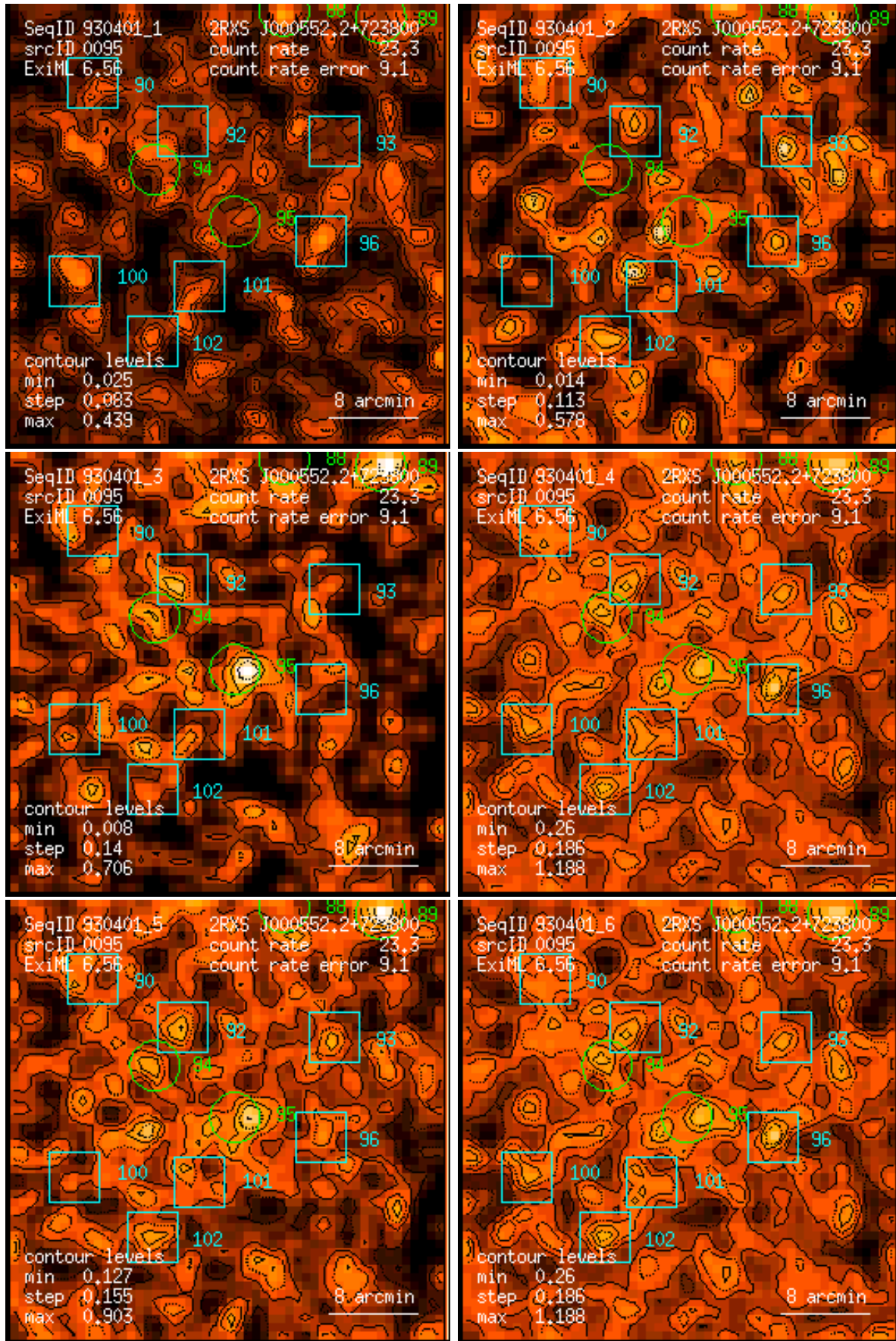
Figure 95: RASS 930401: detection 0095: band rate images, Gaussian filter: (1) PSPC channels 11 – 41, (2) 52 – 90, (3) 91 – 201, (4) 11 – 235, (5) 52 – 201, (6) 11 – 201. Broad band rates in counts/ks. Band rate contour levels in counts/ks/arcmin 2 .
