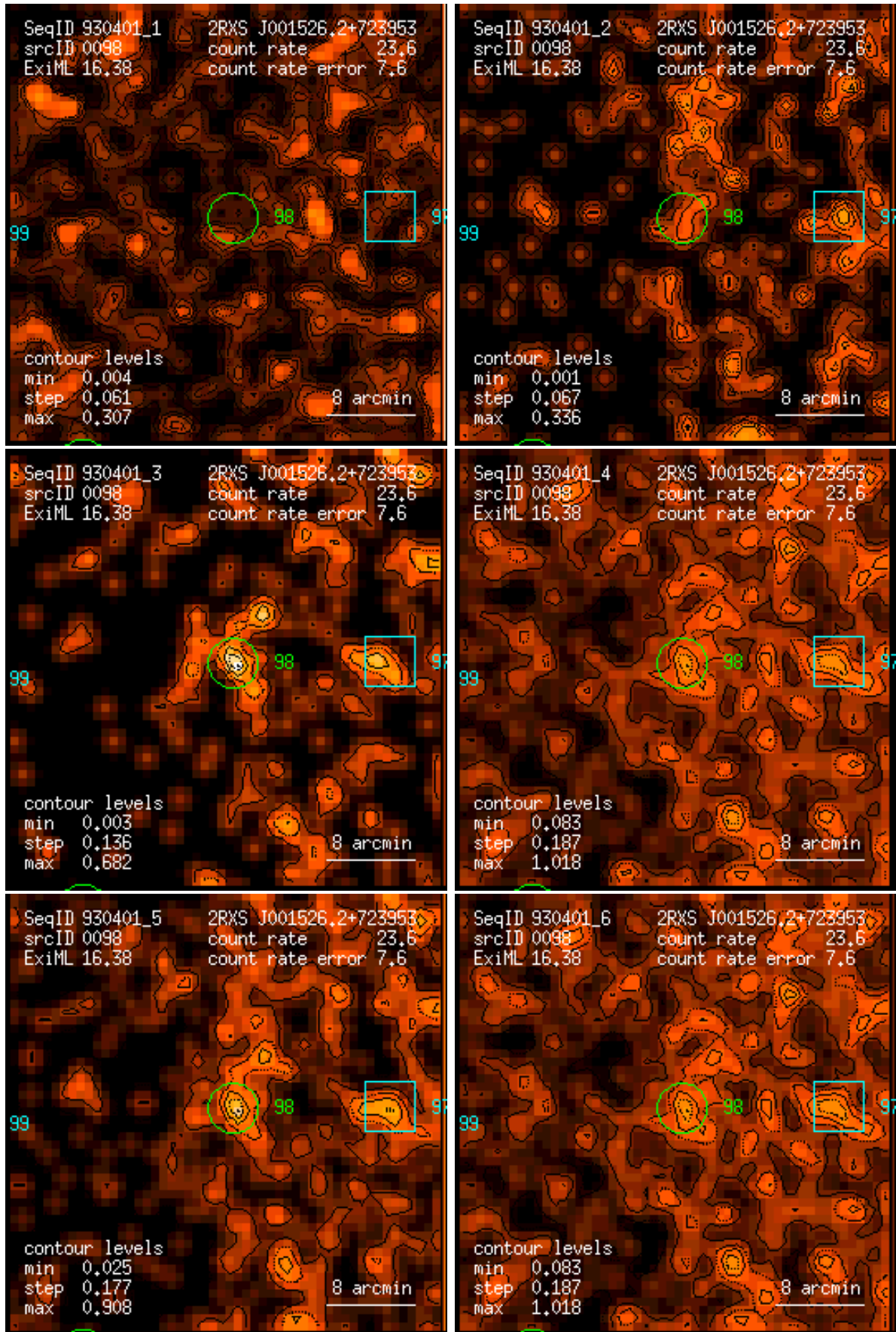
Figure 98: RASS 930401: detection 0098: band rate images, Gaussian filter: (1) PSPC channels 11 – 41, (2) 52 – 90, (3) 91 – 201, (4) 11 – 235, (5) 52 – 201, (6) 11 – 201. Broad band rates in counts/ks. Band rate contour levels in counts/ks/arcmin 2 .
