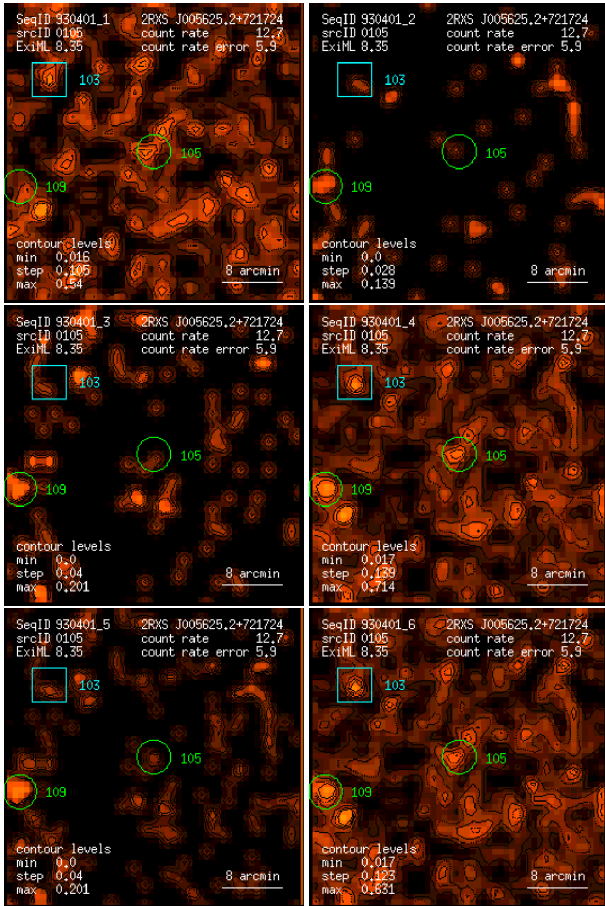
Figure 105: RASS 930401: detection 0105: band rate images, Gaussian filter: (1) PSPC channels 11 – 41, (2) 52 – 90, (3) 91 – 201, (4) 11 – 235, (5) 52 – 201, (6) 11 – 201. Broad band rates in counts/ks. Band rate contour levels in counts/ks/arcmin 2 .
