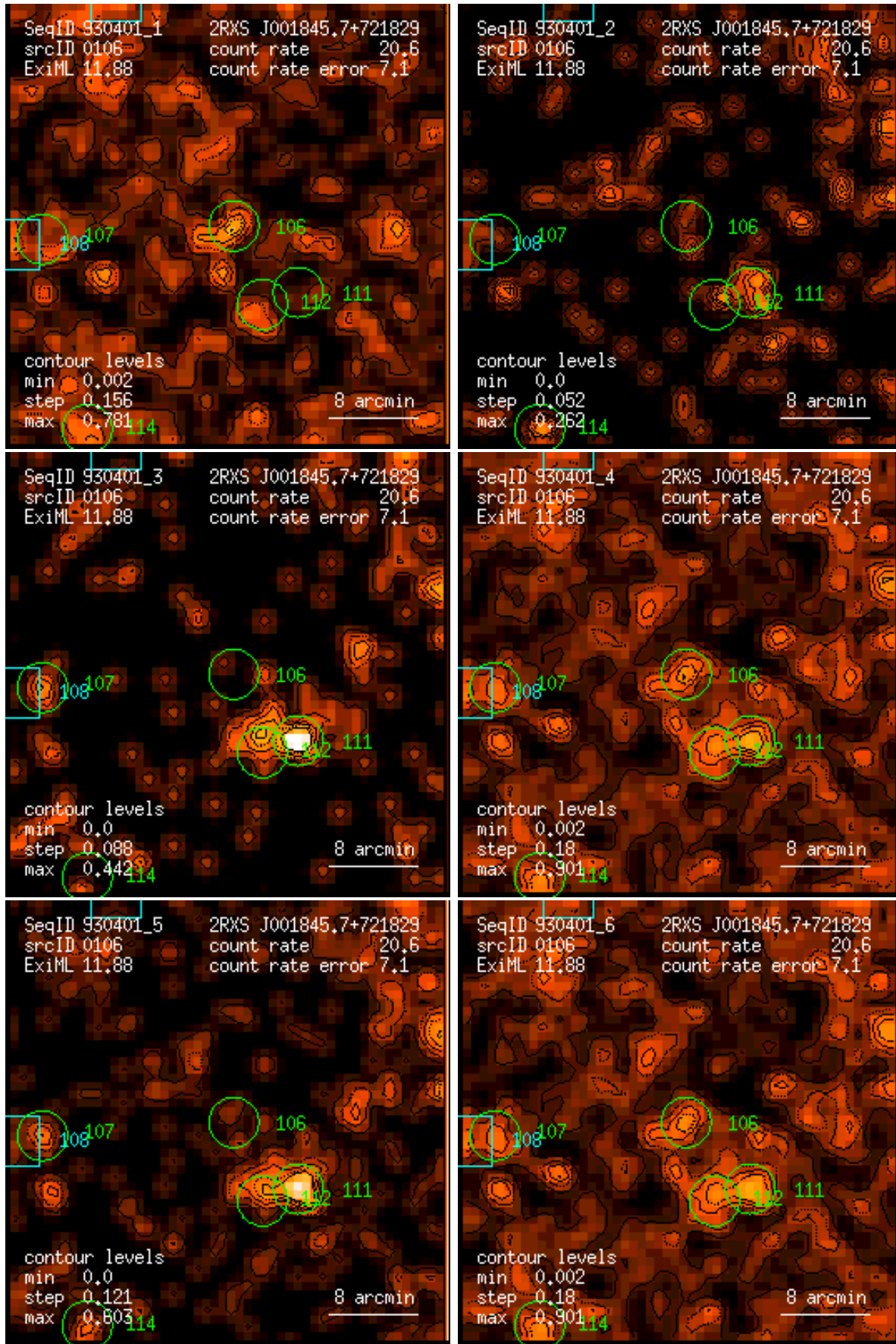
Figure 106: RASS 930401: detection 0106: band rate images, Gaussian filter: (1) PSPP channels 11 – 41, (2) 52 – 90, (3) 91 – 201, (4) 11 – 235, (5) 52 – 201, (6) 11 – 201. Broad band rates in counts/ks. Band rate contour levels in counts/ks/arcmin 2 .
