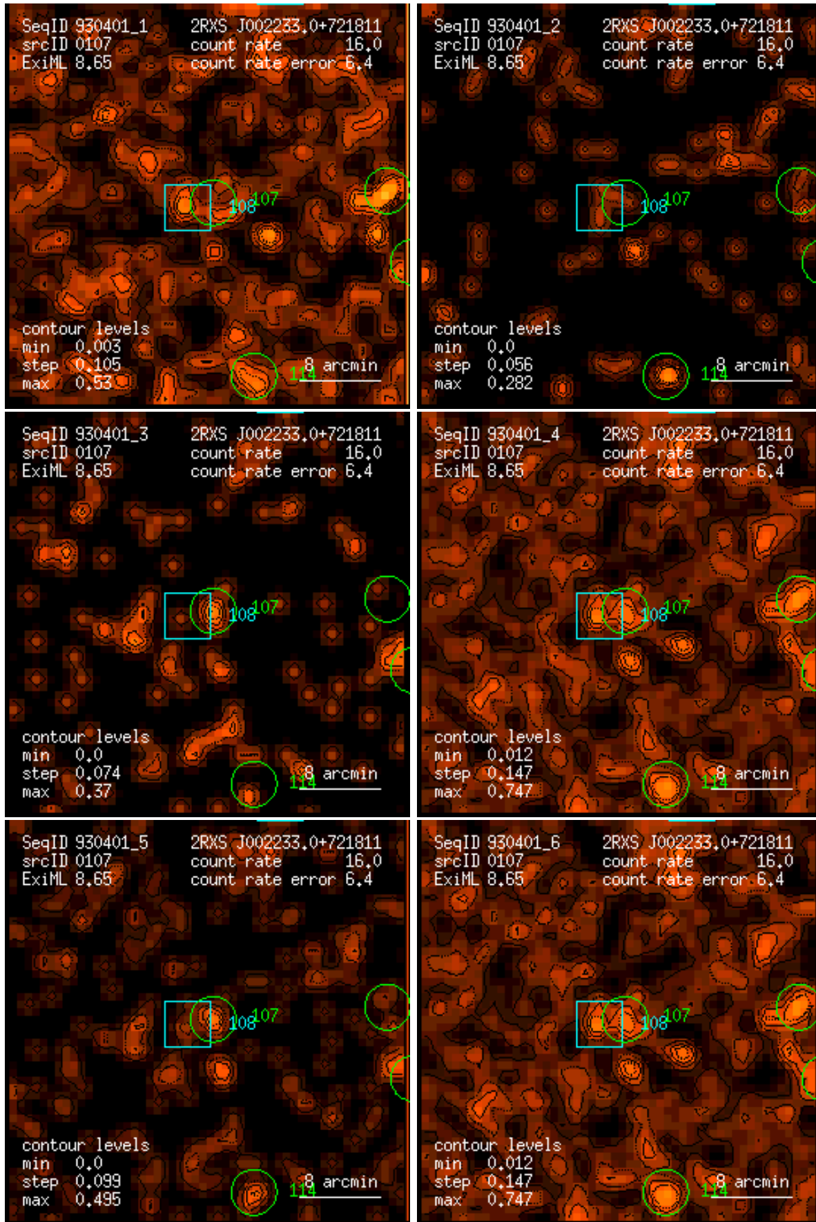
Figure 107: RASS 930401: detection 0107: band rate images, Gaussian filter: (1) PSPC channels 11 – 41, (2) 52 – 90, (3) 91 – 201, (4) 11 – 235, (5) 52 – 201, (6) 11 – 201. Broad band rates in counts/ks. Band rate contour levels in counts/ks/arcmin 2 .
