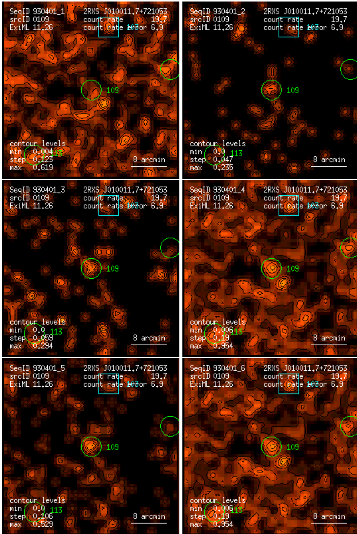
Figure 109: RASS 930401: detection 0109: band rate images, Gaussian filter: (1) PSPC channels 11 – 41, (2) 52 – 90, (3) 91 – 201, (4) 11 – 235, (5) 52 – 201, (6) 11 – 201. Broad band rates in counts/ks. Band rate contour levels in counts/ks/arcmin 2 .
