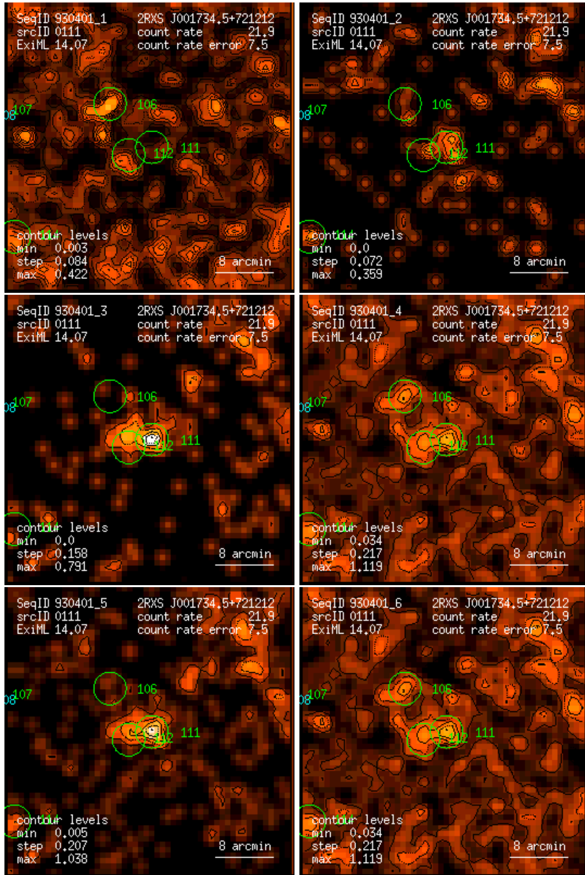
Figure 111: RASS 930401: detection 0111: band rate images, Gaussian filter: (1) PSPC channels 11 – 41, (2) 52 – 90, (3) 91 – 201, (4) 11 – 235, (5) 52 – 201, (6) 11 – 201. Broad band rates in counts/ks. Band rate contour levels in counts/ks/arcmin 2 .
