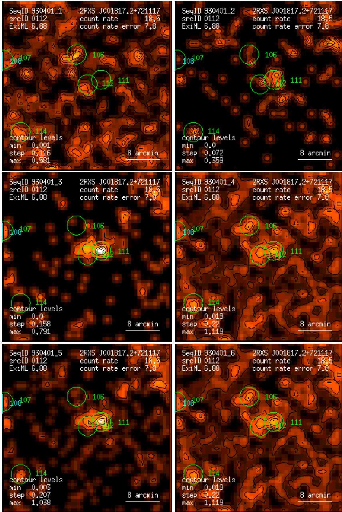
Figure 112: RASS 930401: detection 0112: band rate images, Gaussian filter: (1) PSPC channels 11 – 41, (2) 52 – 90, (3) 91 – 201, (4) 11 – 235, (5) 52 – 201, (6) 11 – 201. Broad band rates in counts/ks. Band rate contour levels in counts/ks/arcmin 2 .
