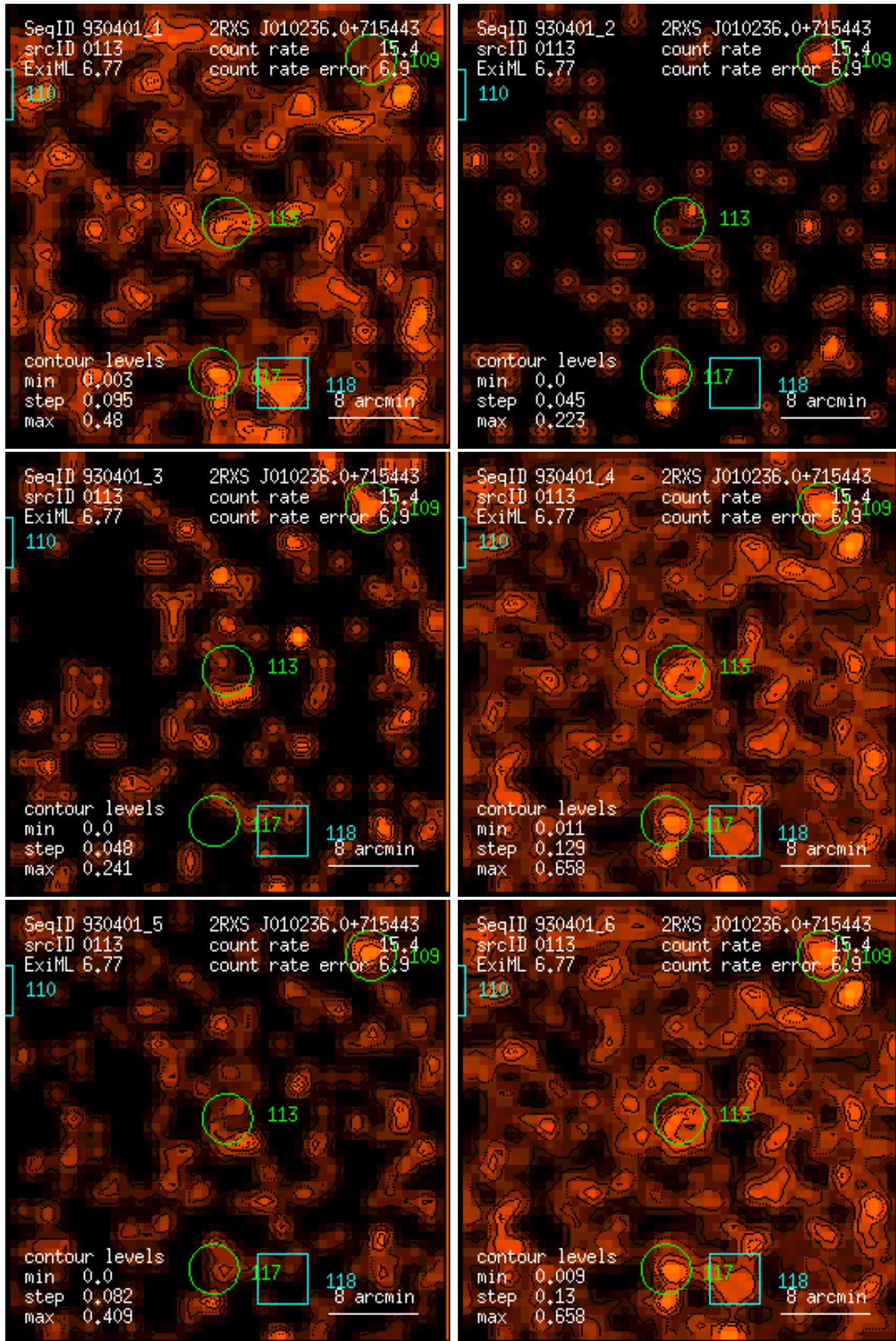
Figure 113: RASS 930401: detection 0113: band rate images, Gaussian filter: (1) PSPC channels 11 – 41, (2) 52 – 90, (3) 91 – 201, (4) 11 – 235, (5) 52 – 201, (6) 11 – 201. Broad band rates in counts/ks. Band rate contour levels in counts/ks/arcmin 2 .
