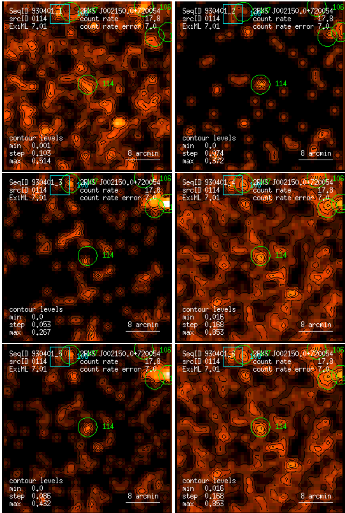
Figure 114: RASS 930401: detection 0114: band rate images, Gaussian filter: (1) PSPC channels 11 – 41, (2) 52 – 90, (3) 91 – 201, (4) 11 – 235, (5) 52 – 201, (6) 11 – 201. Broad band rates in counts/ks. Band rate contour levels in counts/ks/arcmin 2 .
