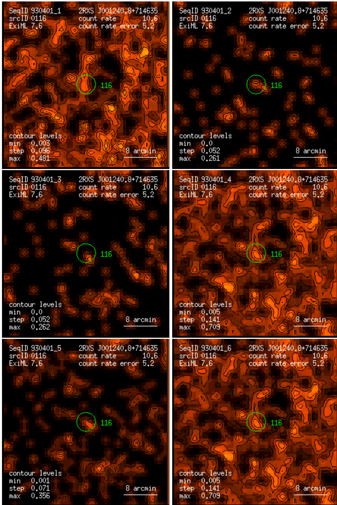
Figure 116: RASS 930401: detection 0116: band rate images, Gaussian filter: (1) PSPC channels 11 – 41, (2) 52 – 90, (3) 91 – 201, (4) 11 – 235, (5) 52 – 201, (6) 11 – 201. Broad band rates in counts/ks. Band rate contour levels in counts/ks/arcmin 2 .
