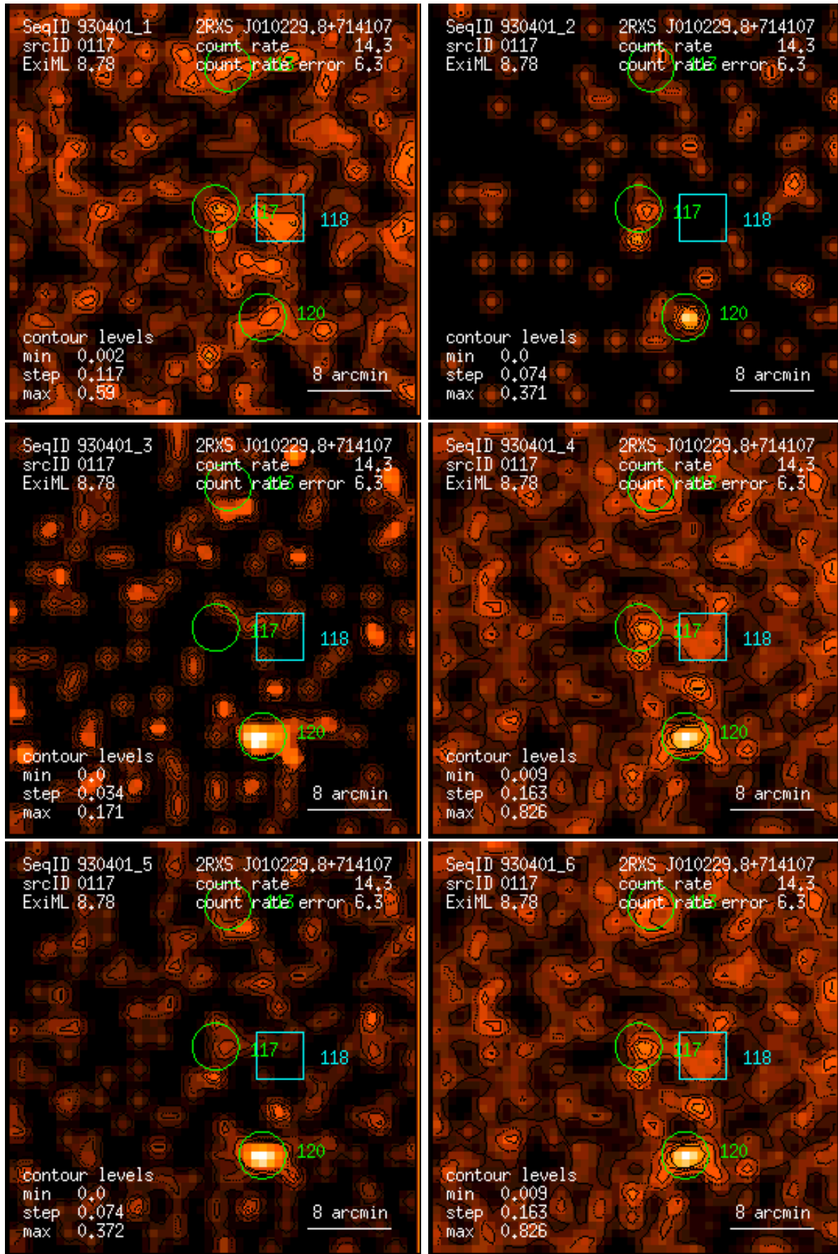
Figure 117: RASS 930401: detection 0117: band rate images, Gaussian filter: (1) PSPC channels 11 – 41, (2) 52 – 90, (3) 91 – 201, (4) 11 – 235, (5) 52 – 201, (6) 11 – 201. Broad band rates in counts/ks. Band rate contour levels in counts/ks/arcmin 2 .
