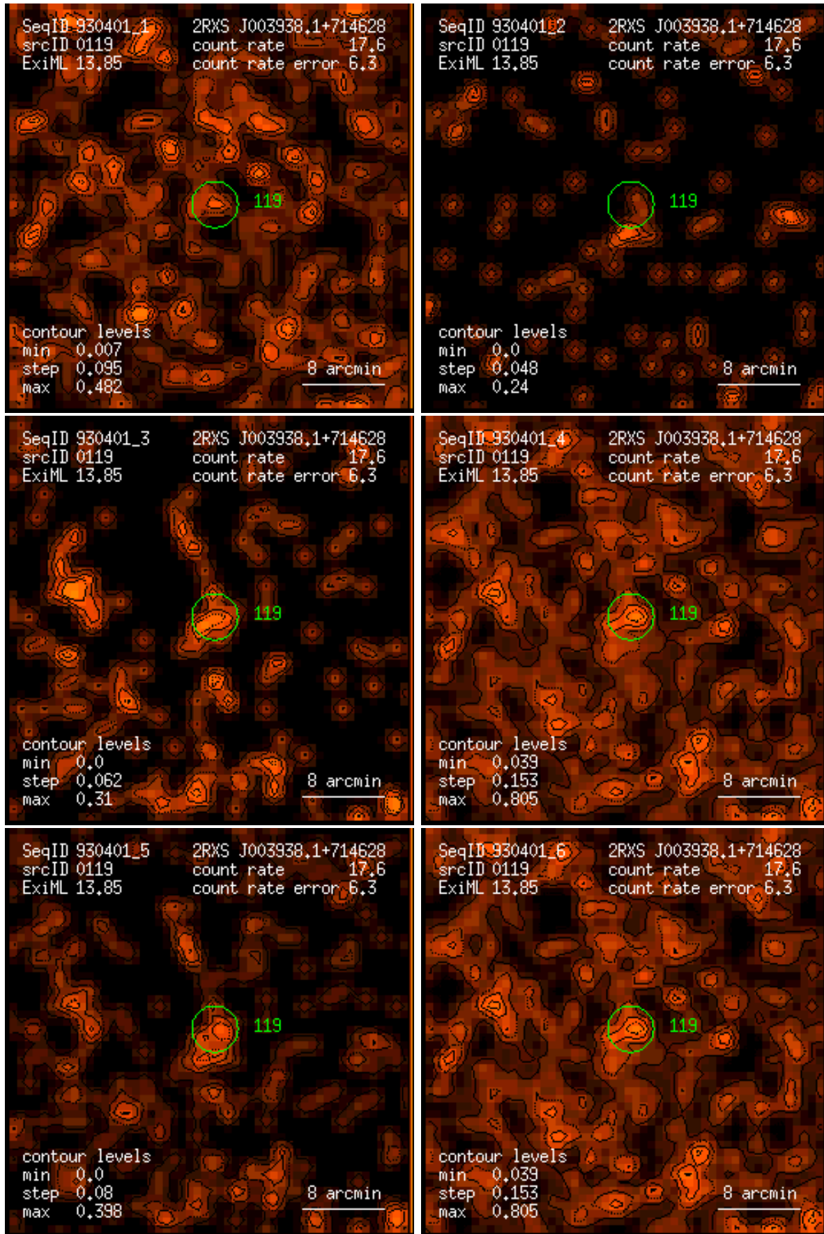
Figure 119: RASS 930401: detection 0119: band rate images, Gaussian filter: (1) PSPC channels 11 – 41, (2) 52 – 90, (3) 91 – 201, (4) 11 – 235, (5) 52 – 201, (6) 11 – 201. Broad band rates in counts/ks. Band rate contour levels in counts/ks/arcmin 2 .
