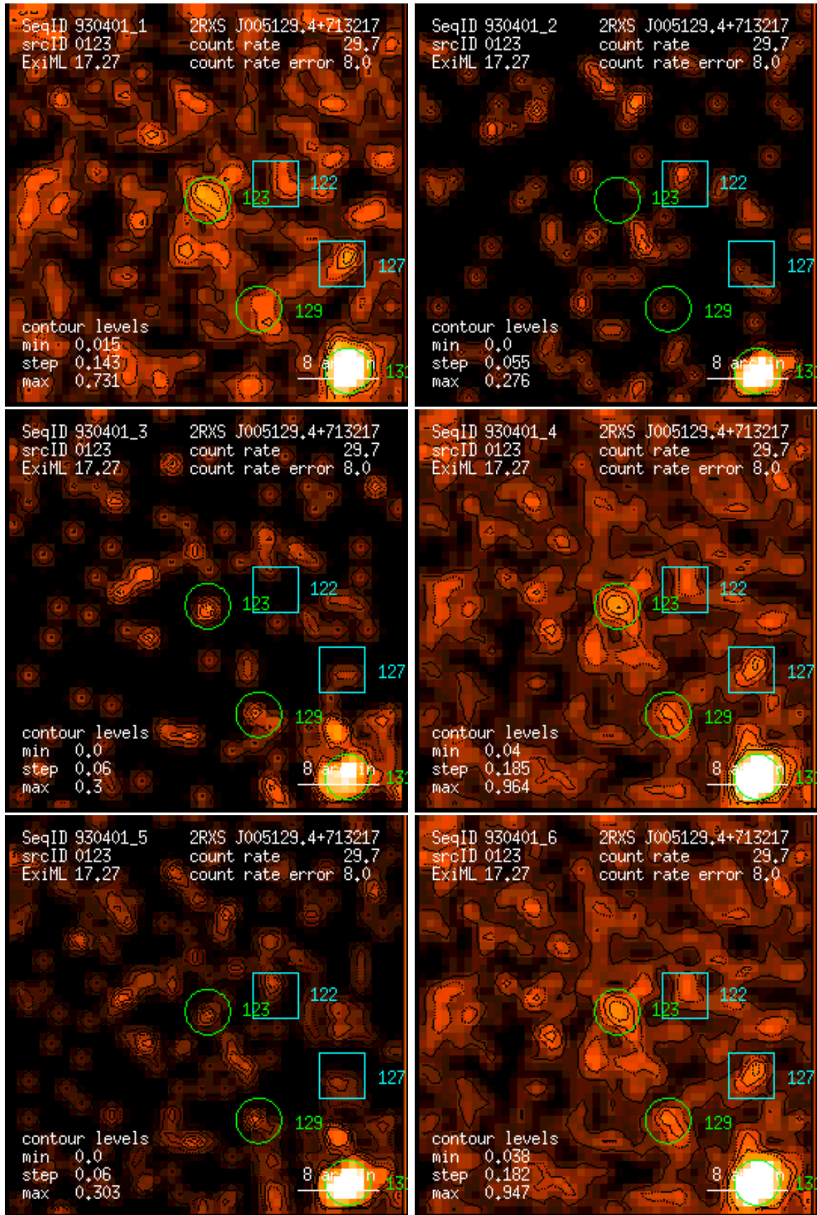
Figure 123: RASS 930401: detection 0123: band rate images, Gaussian filter: (1) PSPC channels 11 – 41, (2) 52 – 90, (3) 91 – 201, (4) 11 – 235, (5) 52 – 201, (6) 11 – 201. Broad band rates in counts/ks. Band rate contour levels in counts/ks/arcmin 2 .
