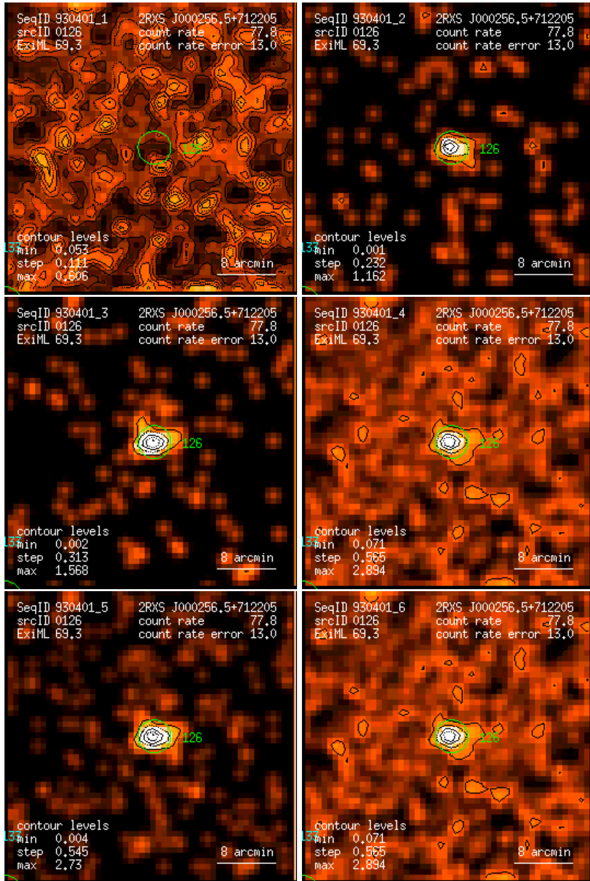
Figure 126: RASS 930401: detection 0126: band rate images, Gaussian filter: (1) PSPC channels 11 – 41, (2) 52 – 90, (3) 91 – 201, (4) 11 – 235, (5) 52 – 201, (6) 11 – 201. Broad band rates in counts/ks. Band rate contour levels in counts/ks/arcmin 2 .
