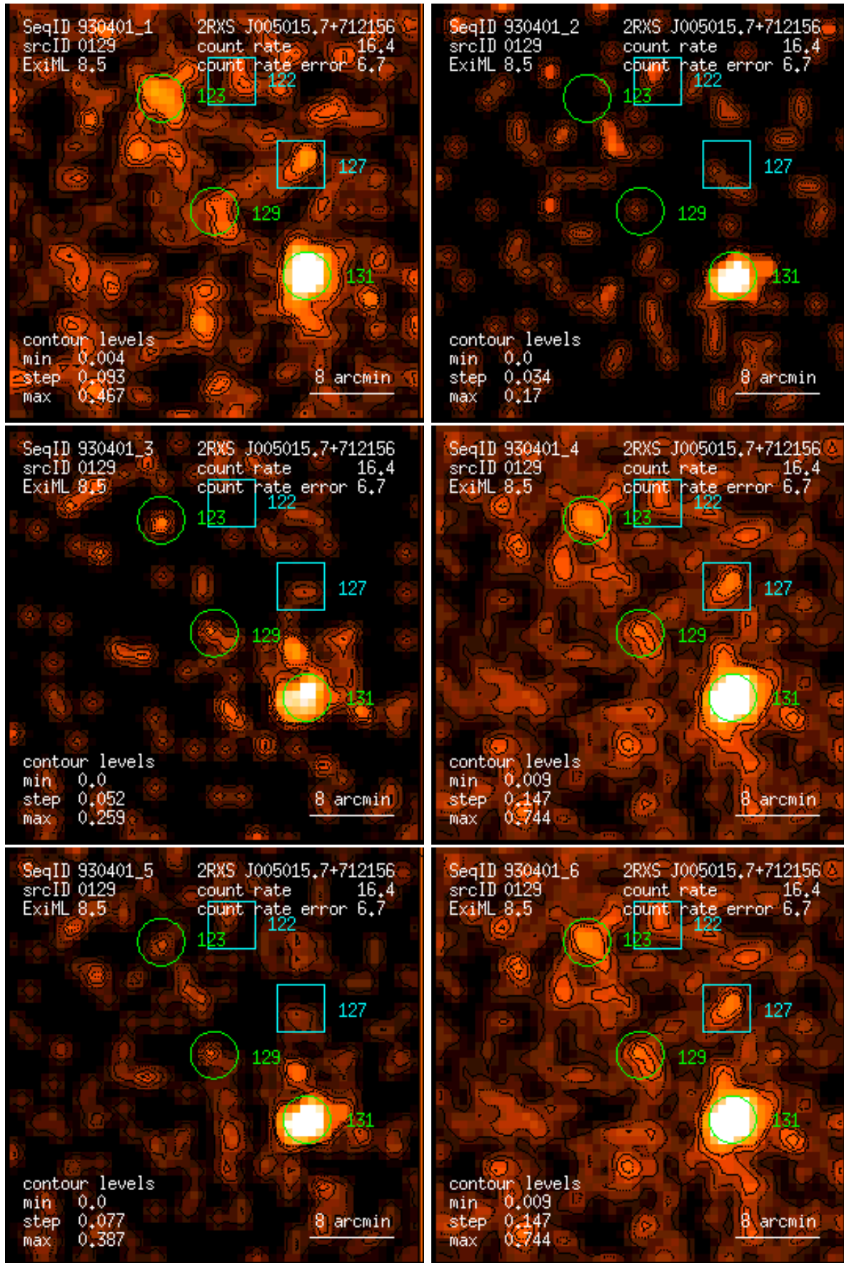
Figure 129: RASS 930401: detection 0129: band rate images, Gaussian filter: (1) PSPC channels 11 – 41, (2) 52 – 90, (3) 91 – 201, (4) 11 – 235, (5) 52 – 201, (6) 11 – 201. Broad band rates in counts/ks. Band rate contour levels in counts/ks/arcmin 2 .
