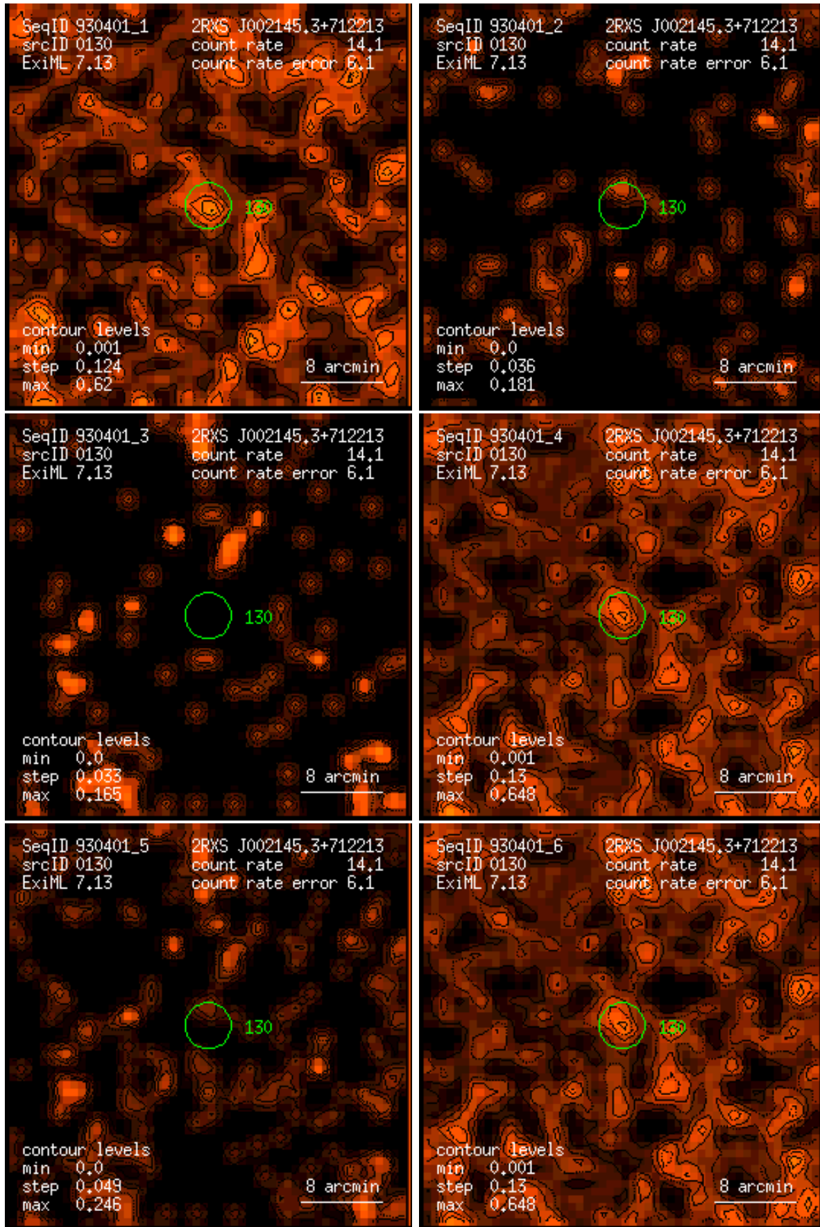
Figure 130: RASS 930401: detection 0130: band rate images, Gaussian filter: (1) PSPC channels 11 – 41, (2) 52 – 90, (3) 91 – 201, (4) 11 – 235, (5) 52 – 201, (6) 11 – 201. Broad band rates in counts/ks. Band rate contour levels in counts/ks/arcmin 2 .
